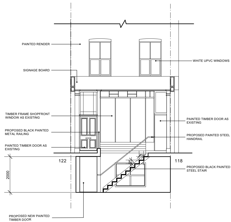
01/2023 PROPOSED SECTION AA 1:100
