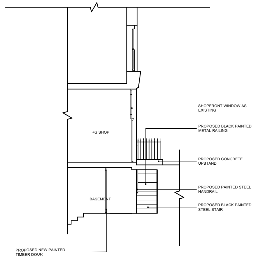
01/2023 PROPOSED SECTION BB 1:100
