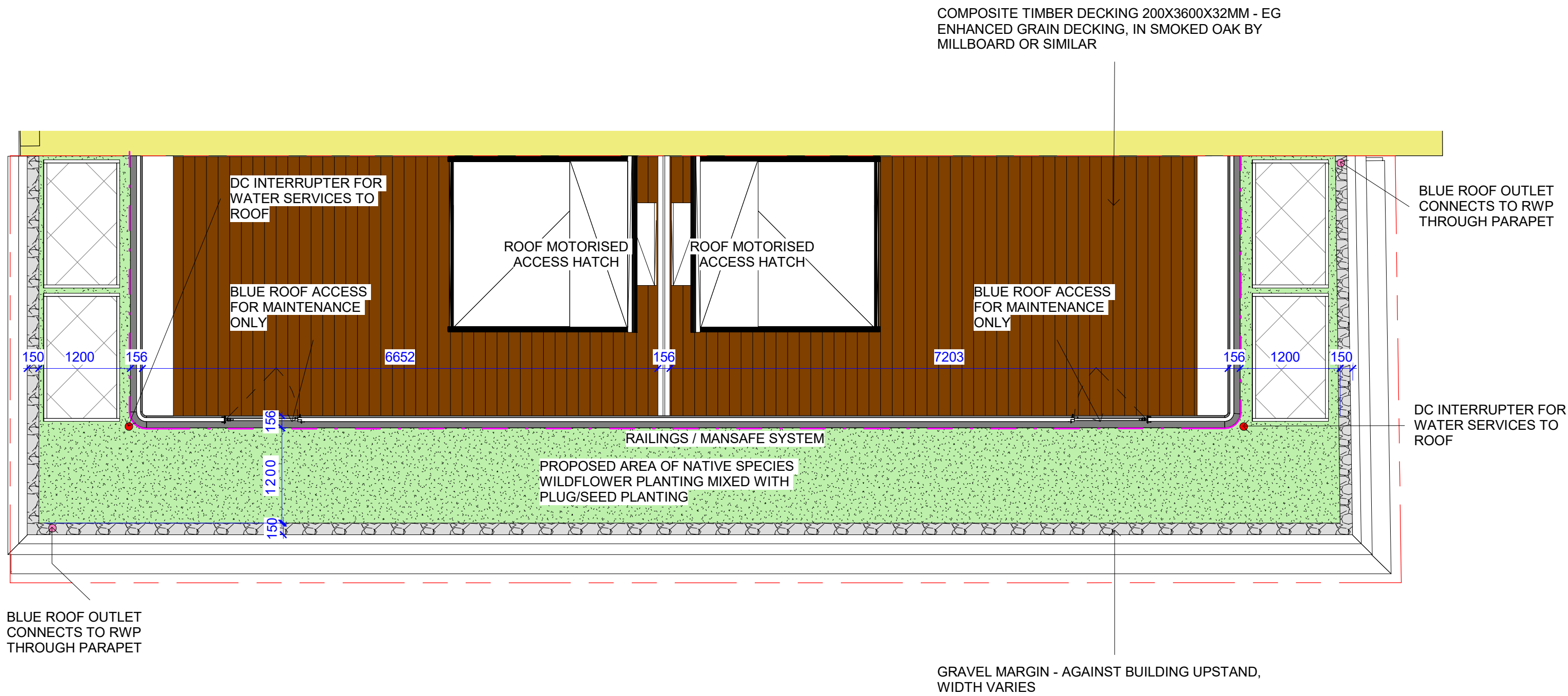
1 Landscaping Plan - Roof Level 1 : 50
