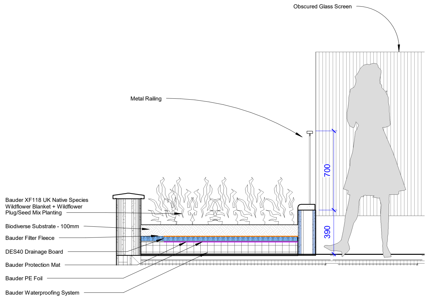
2 Green Roof Typical Section 1 : 20
