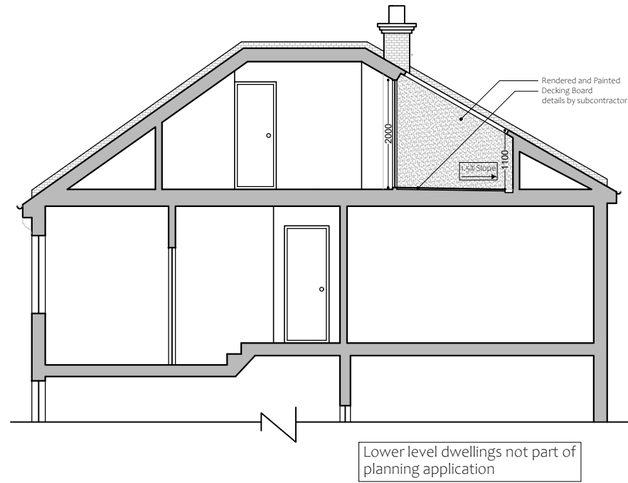
② Proposed Cross Section
