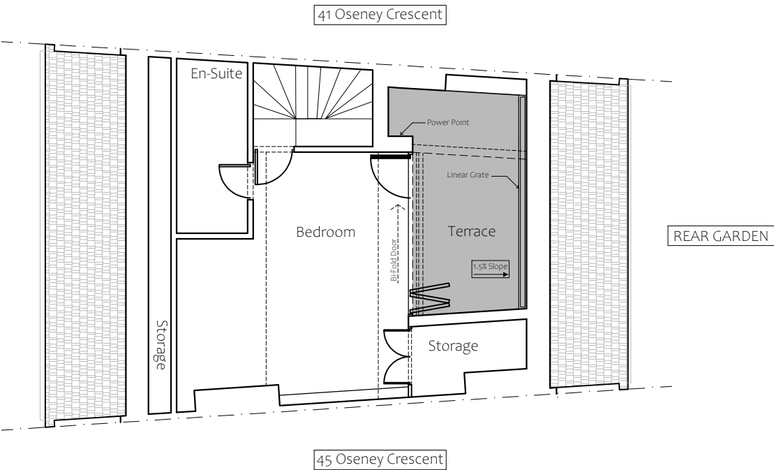
1 Proposed Loft Floor Plan Layout
