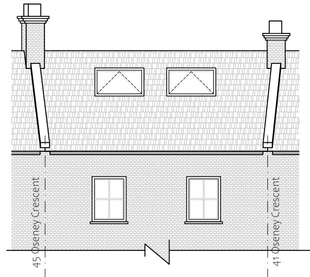
② Existing Rear Elevation
