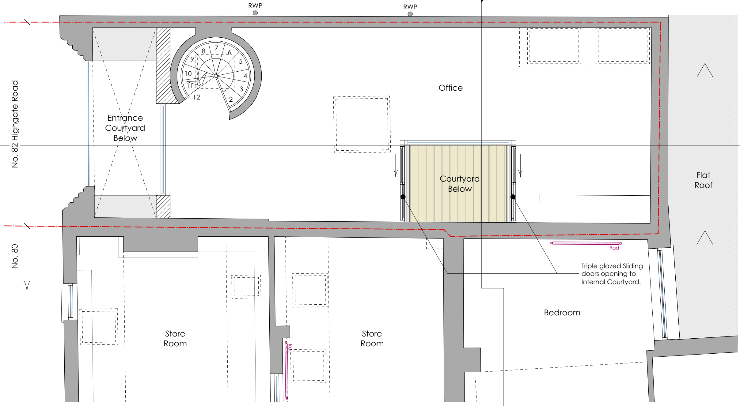
1 Proposed First Floor Plan Scale: 1:50
