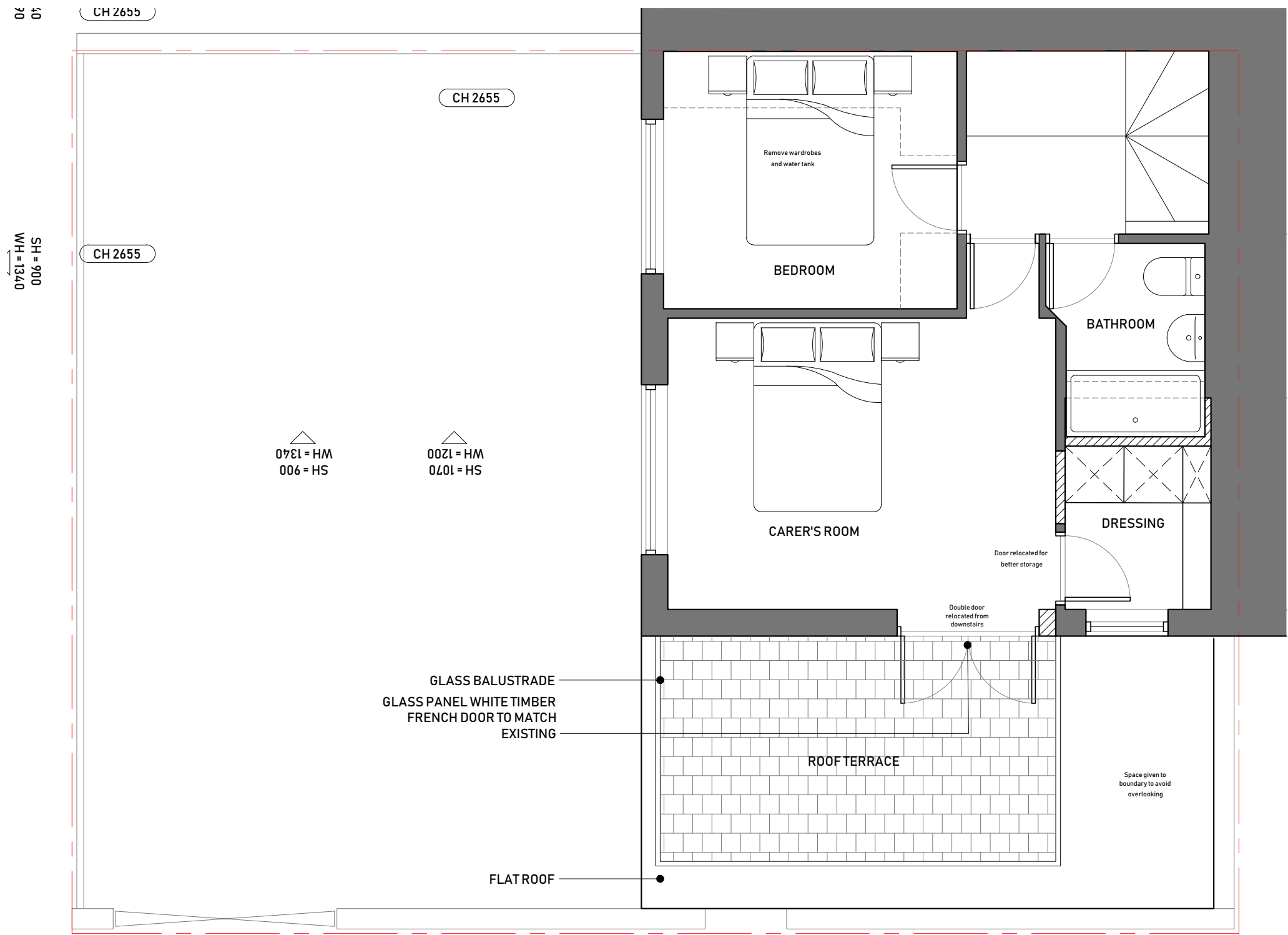
Proposed First Floor Plan Scale 1:50 @ A3
