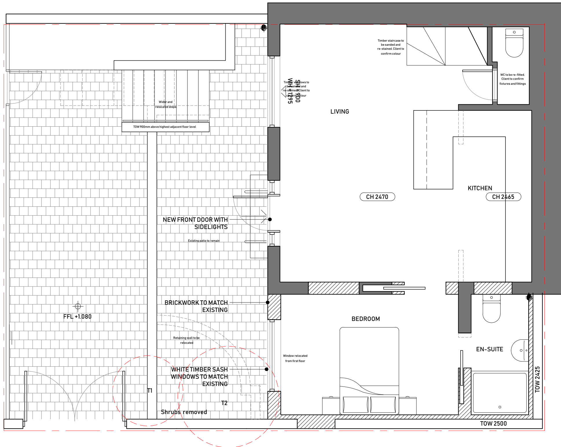
Proposed Ground Floor Plan Scale 1:50 @ A3
