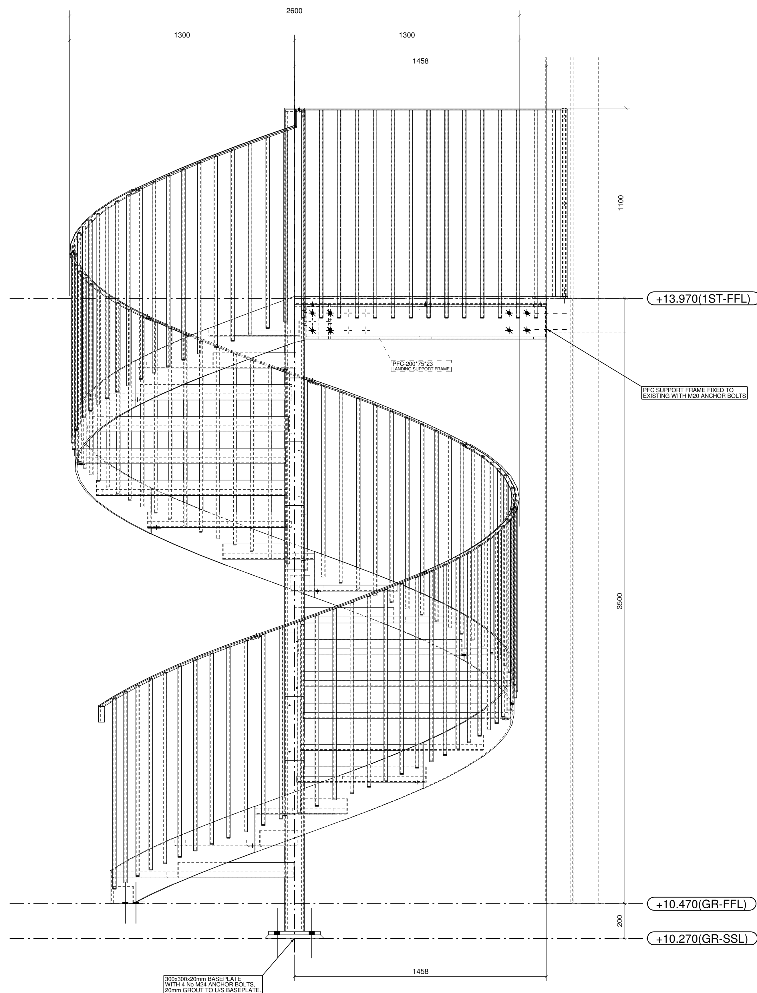
Section A (FROM GA-CC-SS-01)
