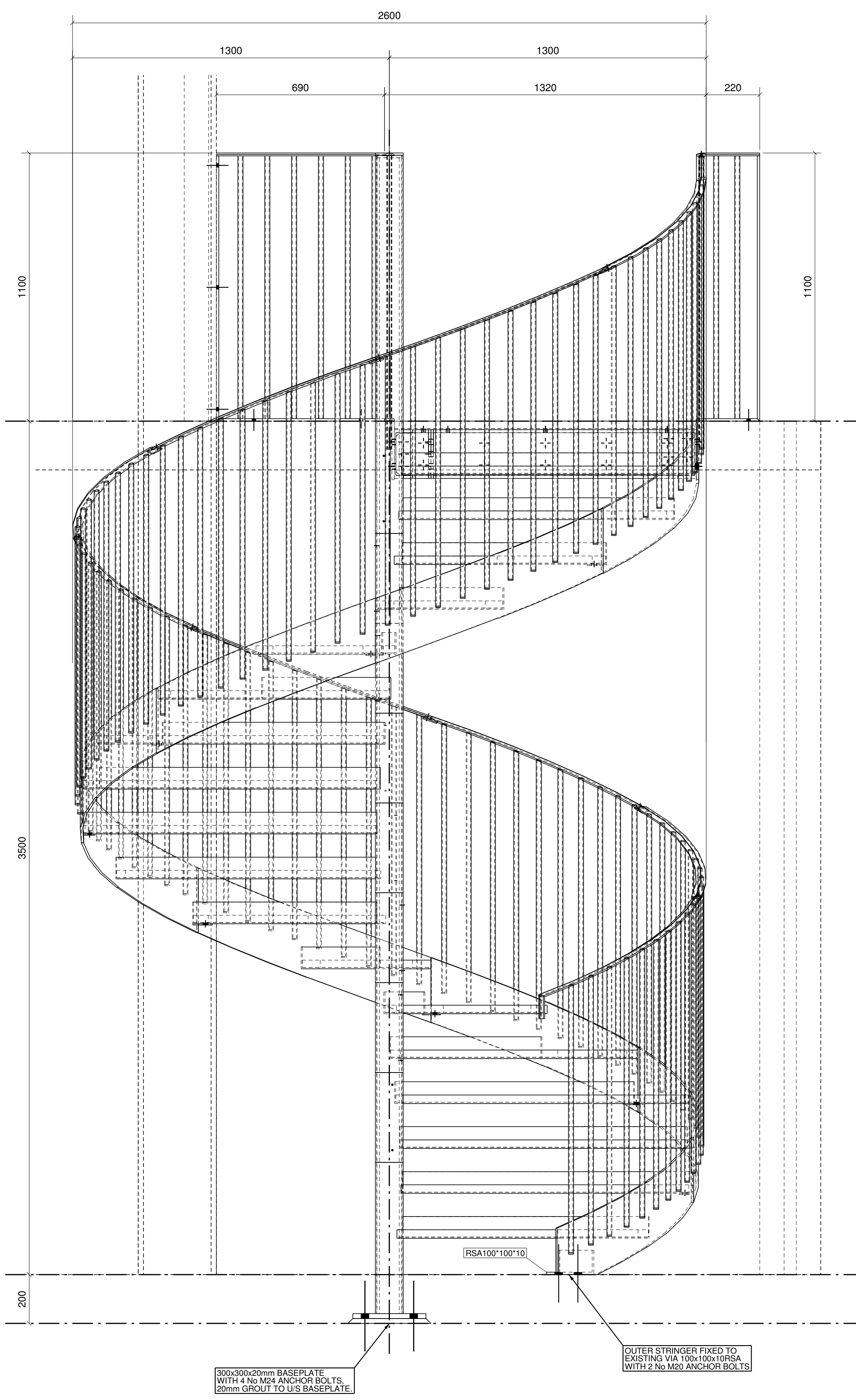
Section B (FROM GA-CC-SS-01)
