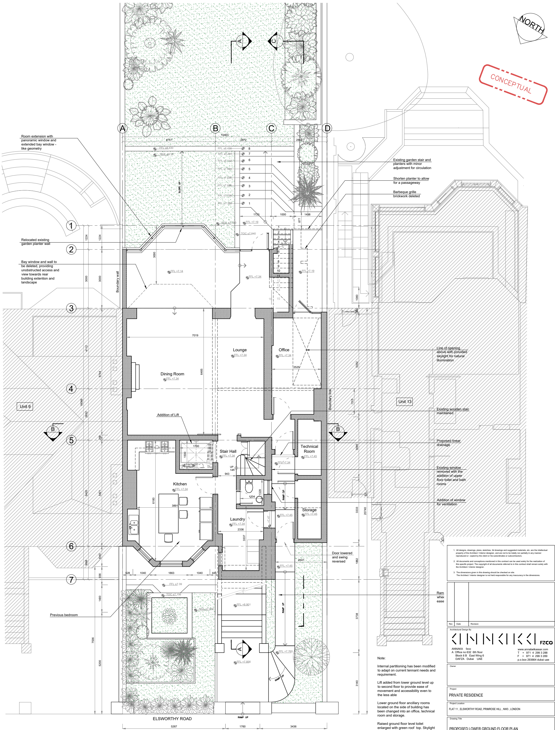
PROPOSED LOWER GROUND FLOOR PLAN SCALE: 1:100 on A3
