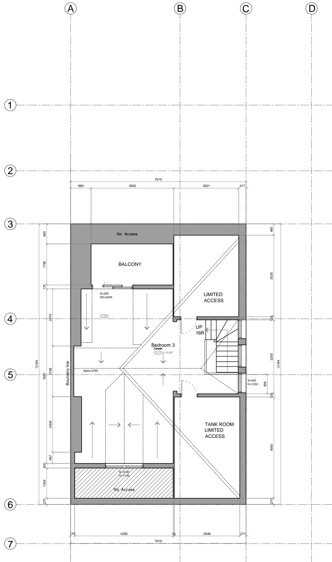
Existing THIRD FLOOR PLAN SCALE: 1:100 on A3
