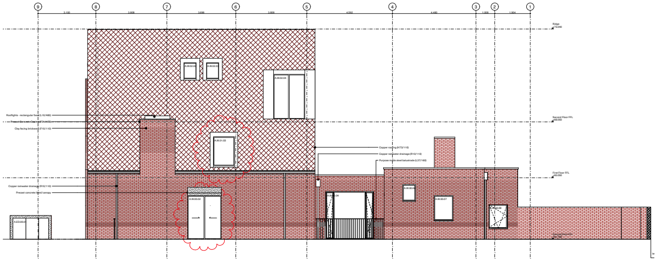
West Elevation - Consented
