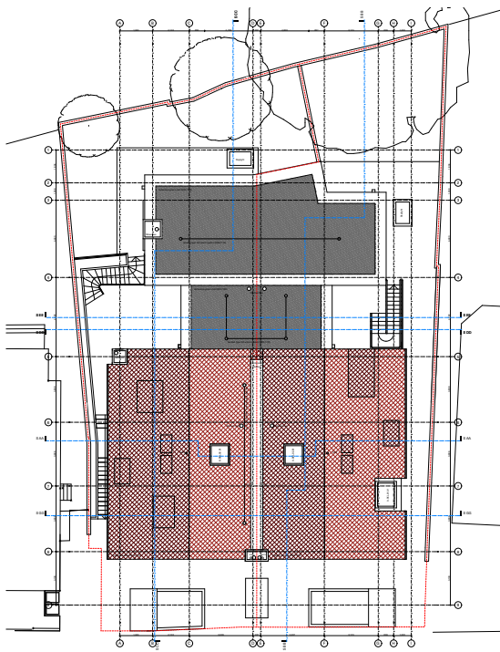
Roof Plan - Consented
