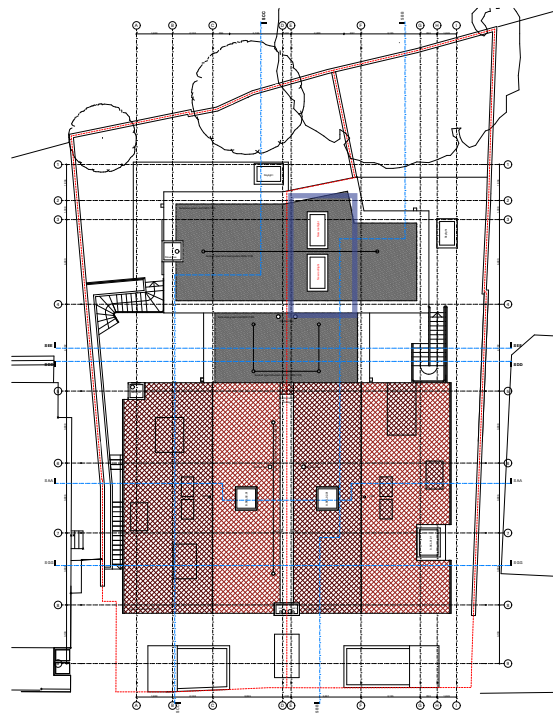
Roof Plan - Proposed
