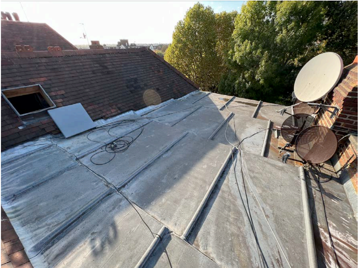
4 - Existing roof looking west towards the gardens
