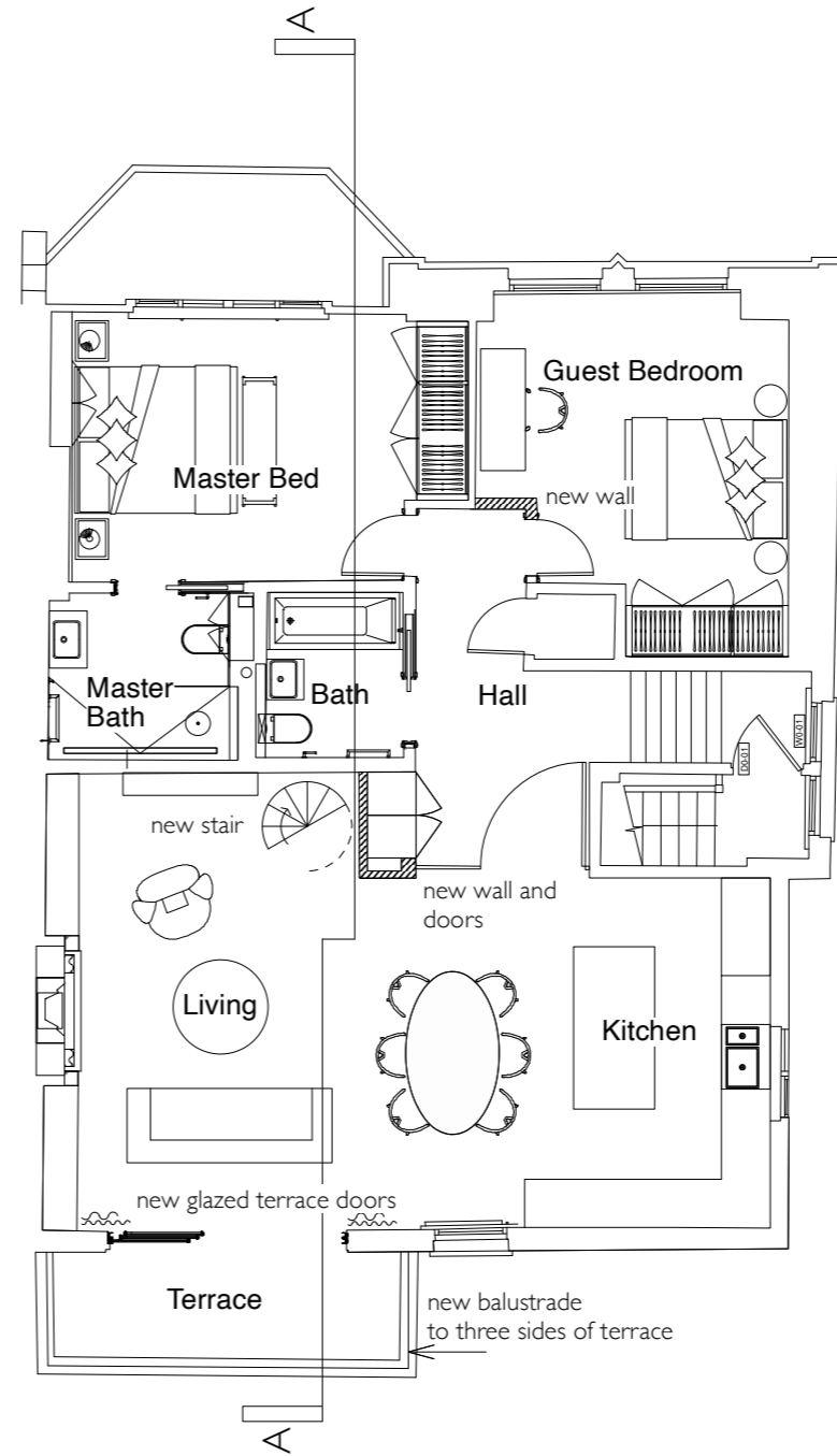
2 Proposed Plan 1:100
