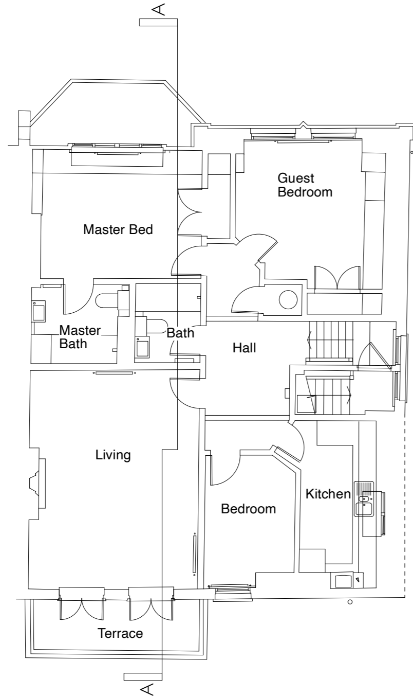
1 Existing Plan 1:100
