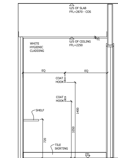
B ACCESSIBLE WC ELEVATION B 1:20
