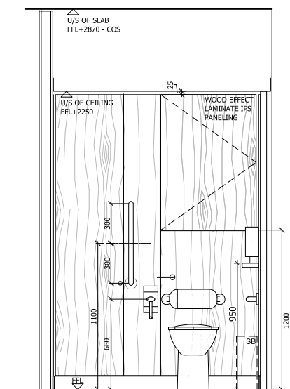
D ACCESSIBLE WC ELEVATION D 1:20
