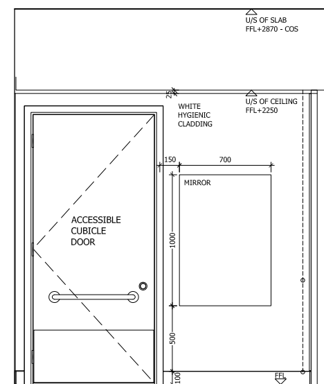
C ACCESSIBLE WC ELEVATION C 1:20
