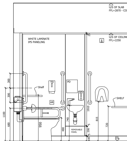
A ACCESSIBLE WC ELEVATION A 1:20
