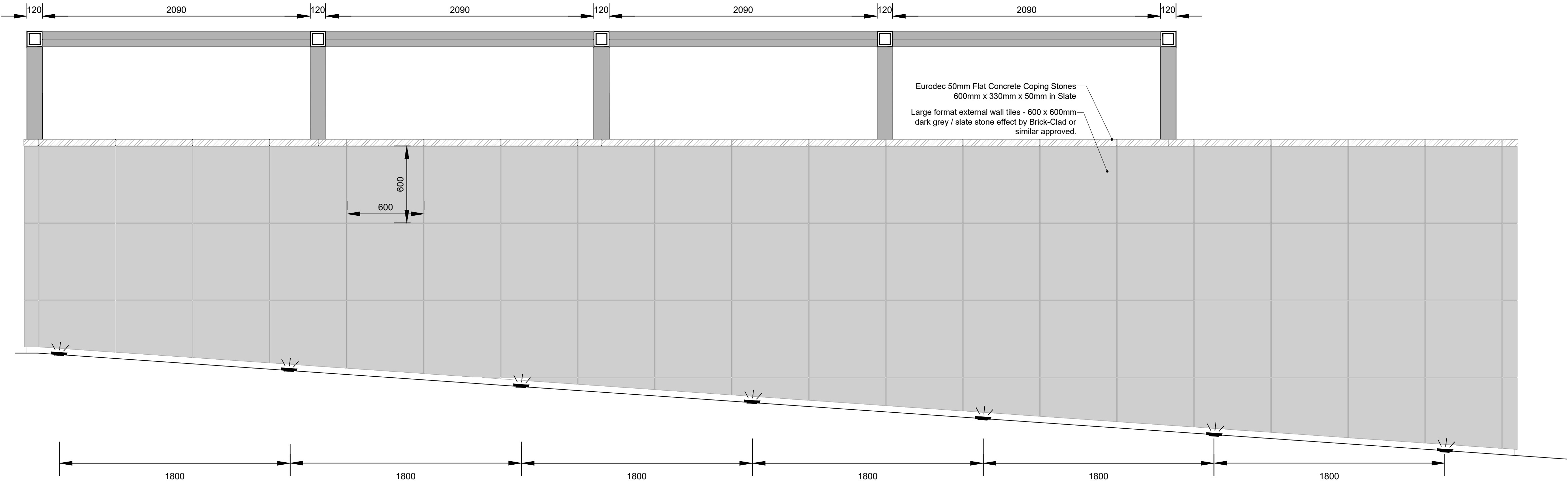
Section C 1:20
