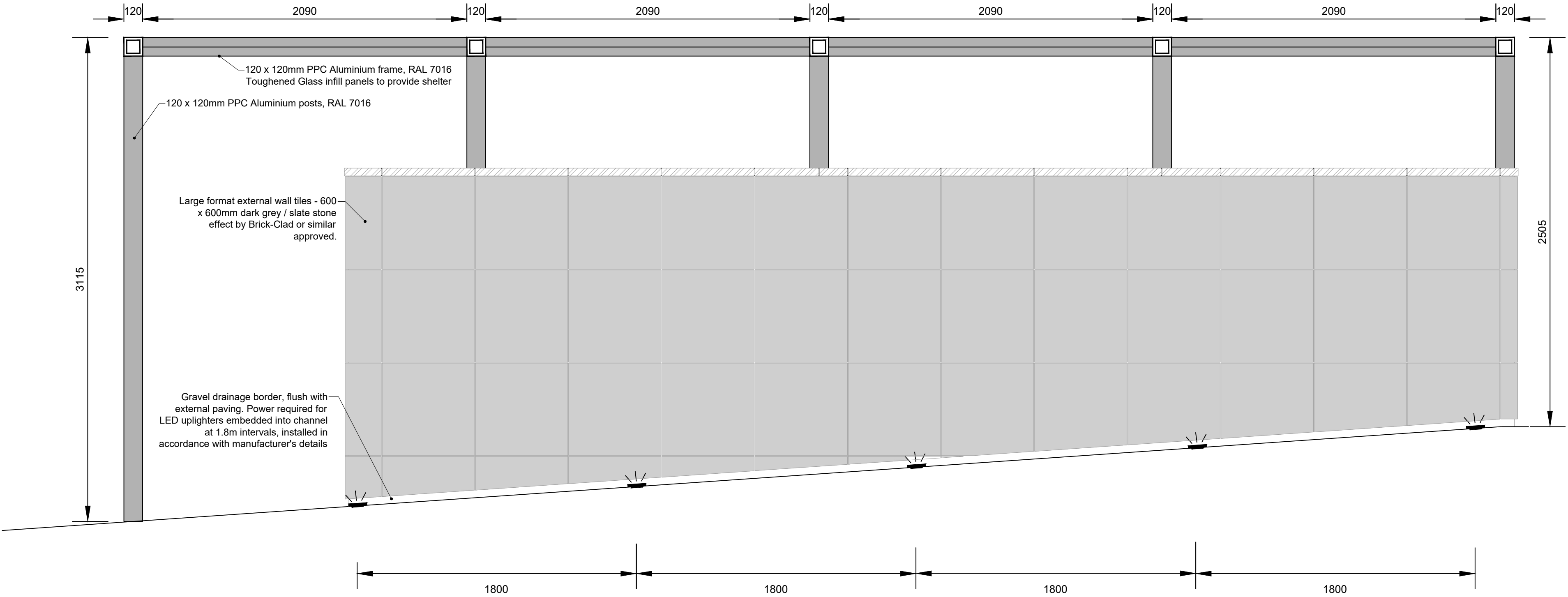
Section B 1:20
