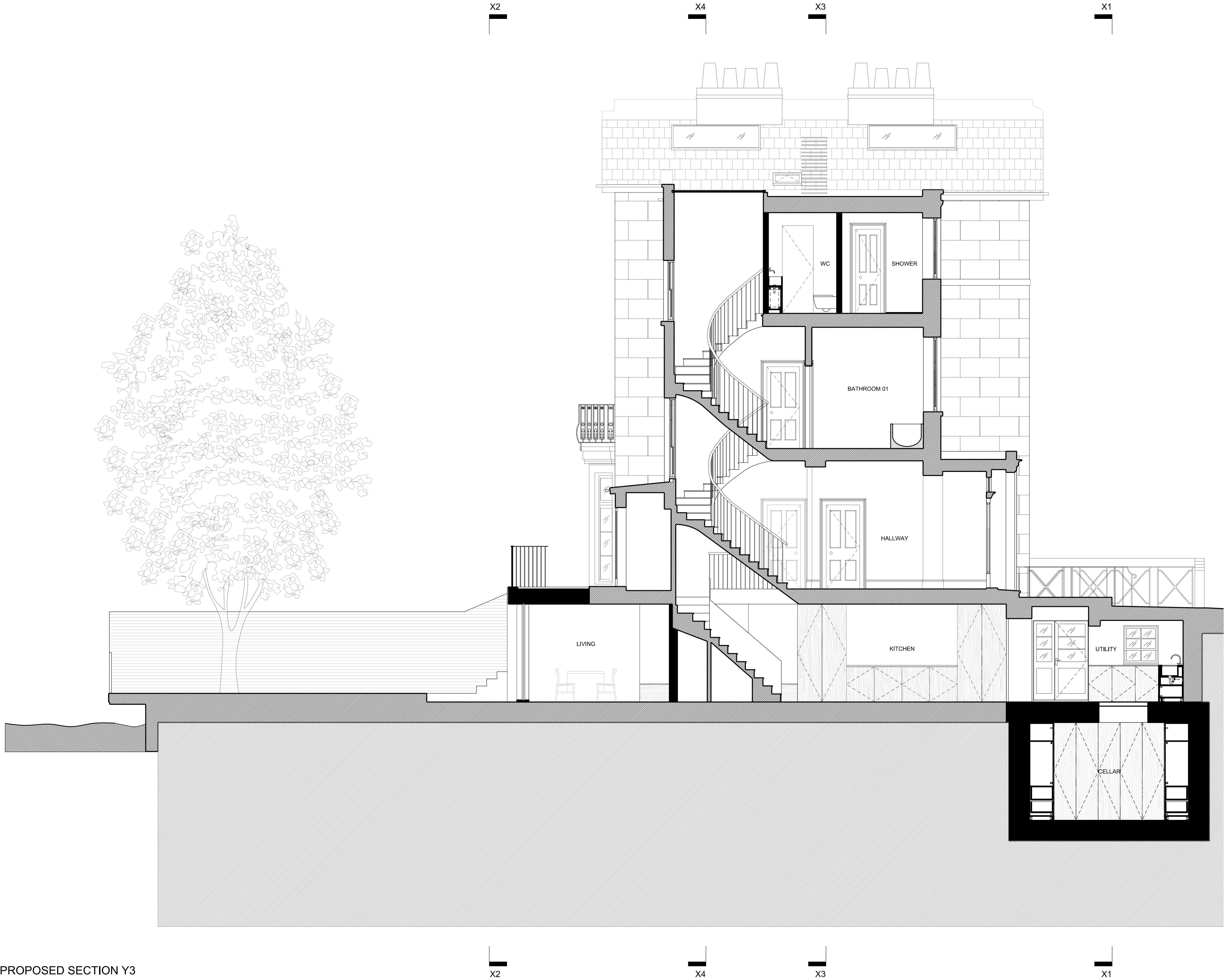
PROPOSED SECTION Y3
