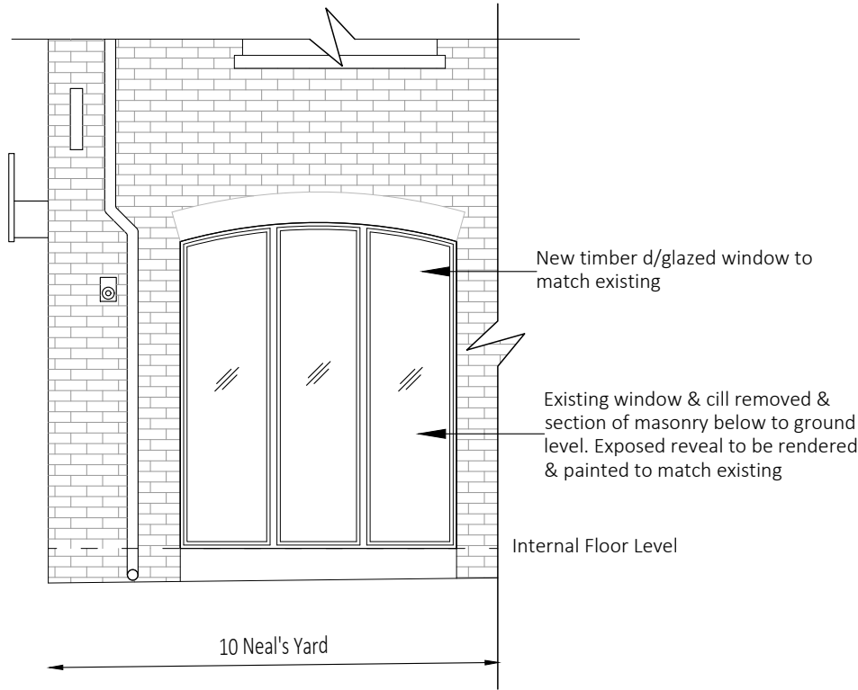
North Elevation
