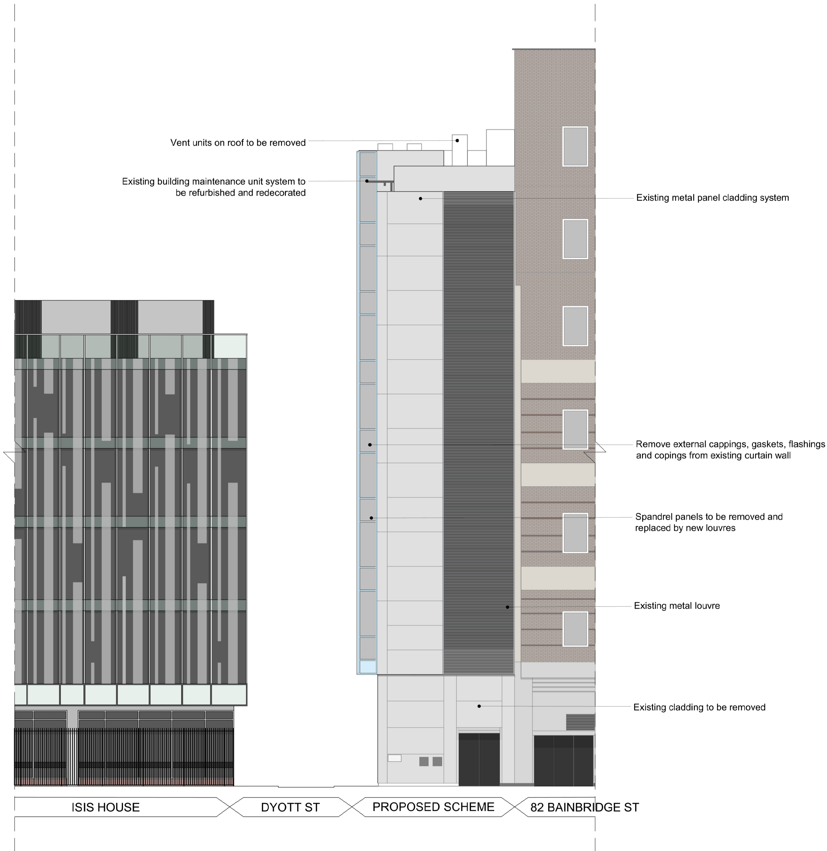
1 Existing Bainbridge Street Elevation 1 : 100
