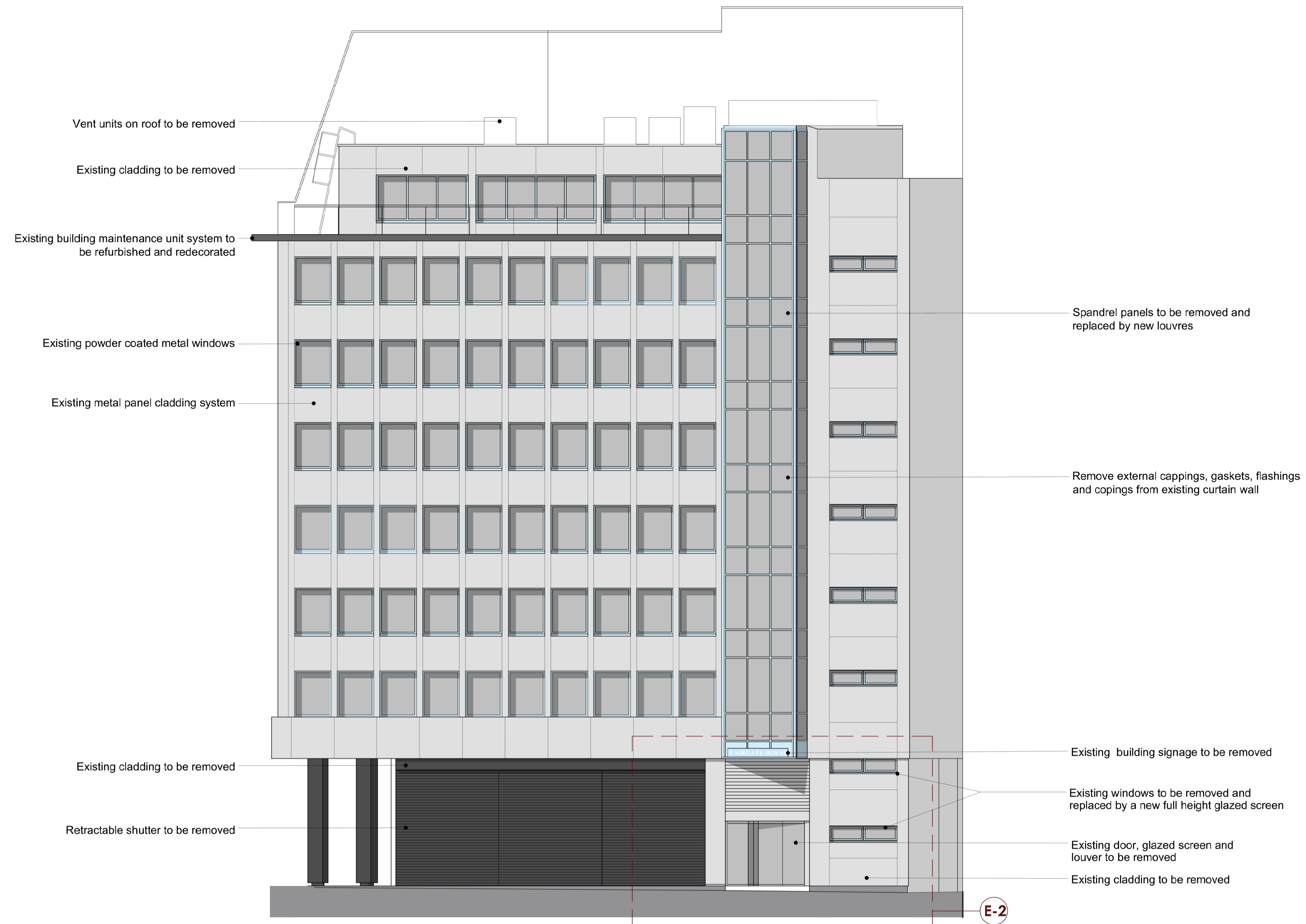
1 Existing Dyott Street Elevation 1 : 100
