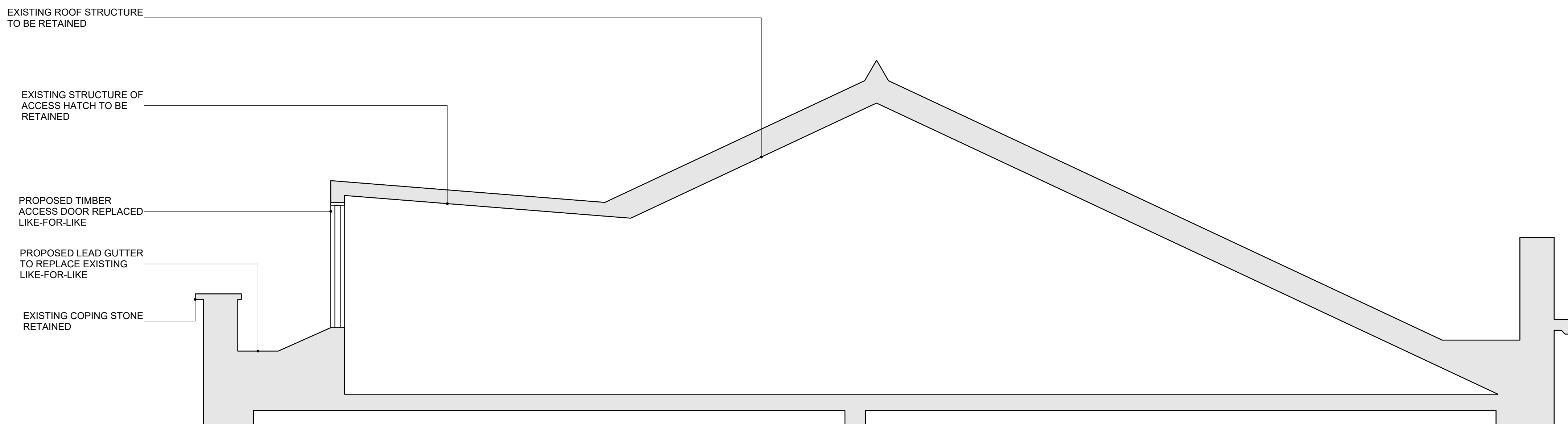
03 ROOF SECTION DETAILS 1:20 @ A1
