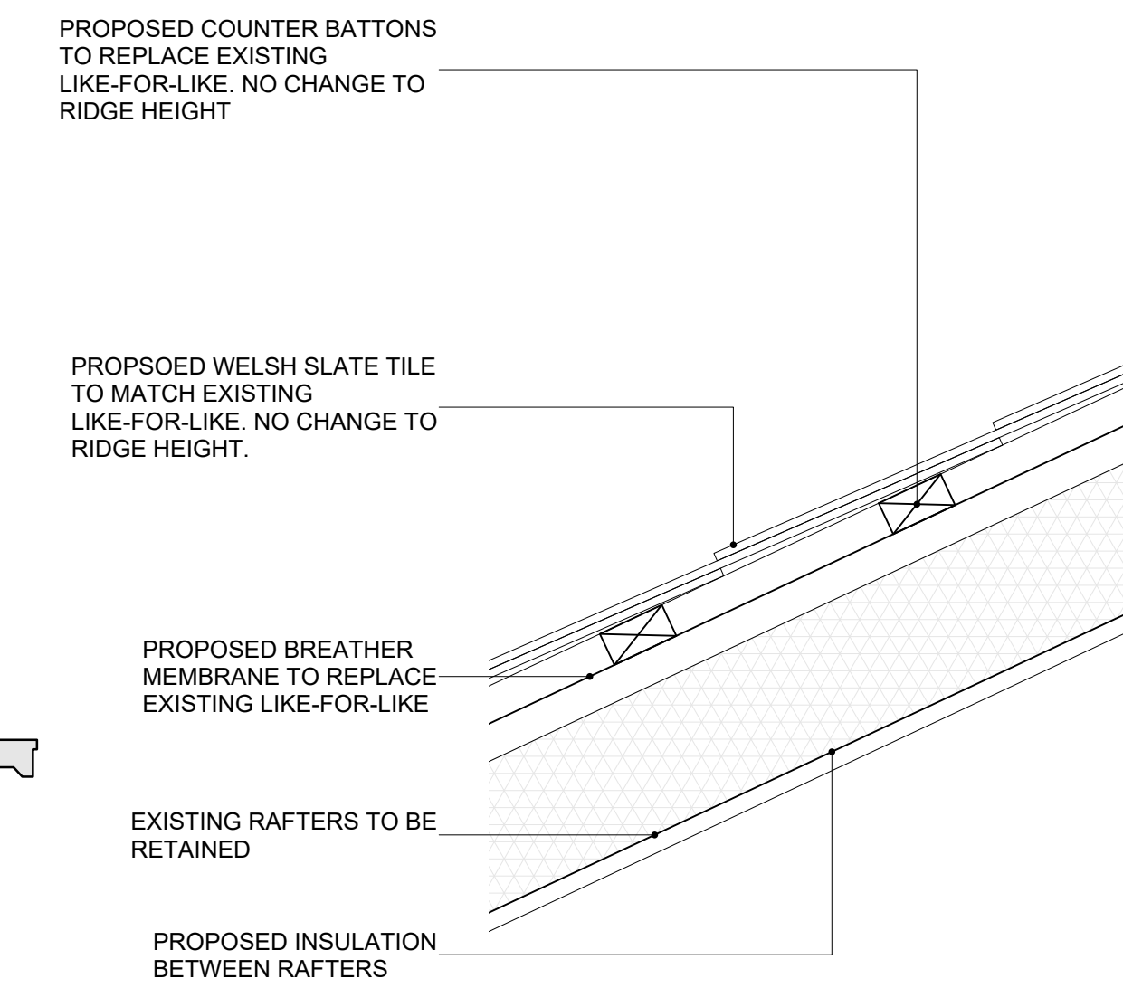
04 ROOF BUILD UP DETAIL 1:5 @ A1
