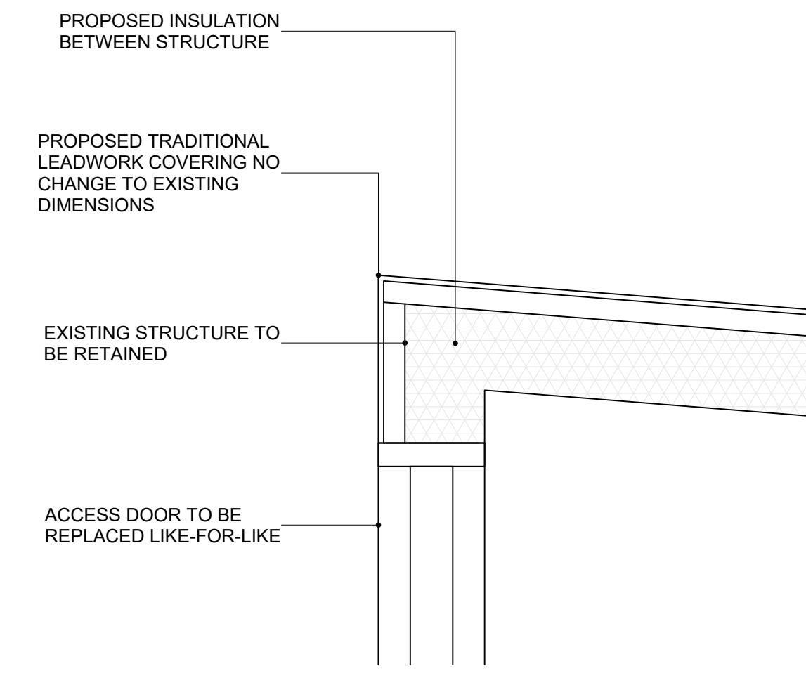
02 ACCESS HATCH BUILD UP DETAIL 1:5 @ A1
