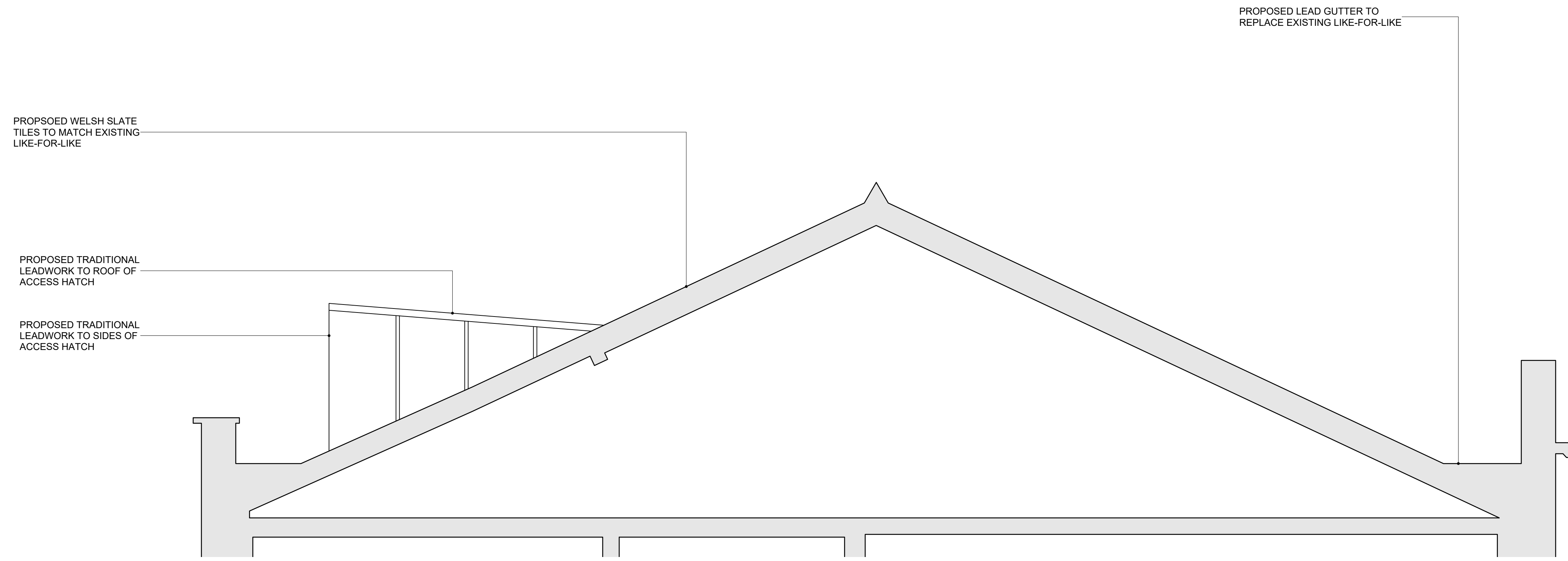
01 ROOF ELEVATION DETAILS 1:20 @ A1
