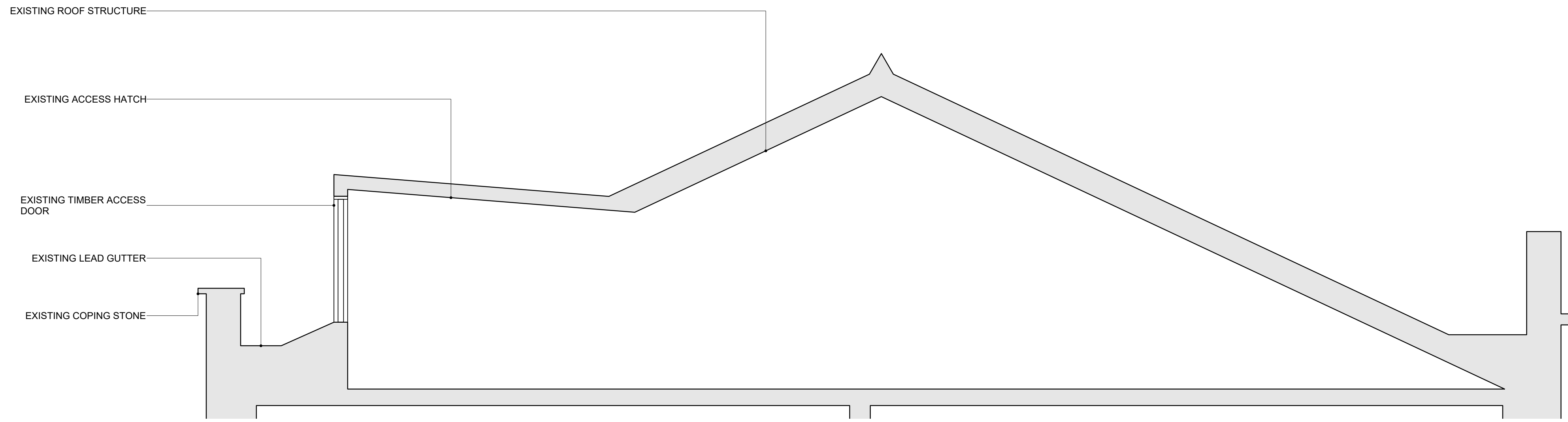
03 ROOF SECTION DETAILS 1:20 @ A1
