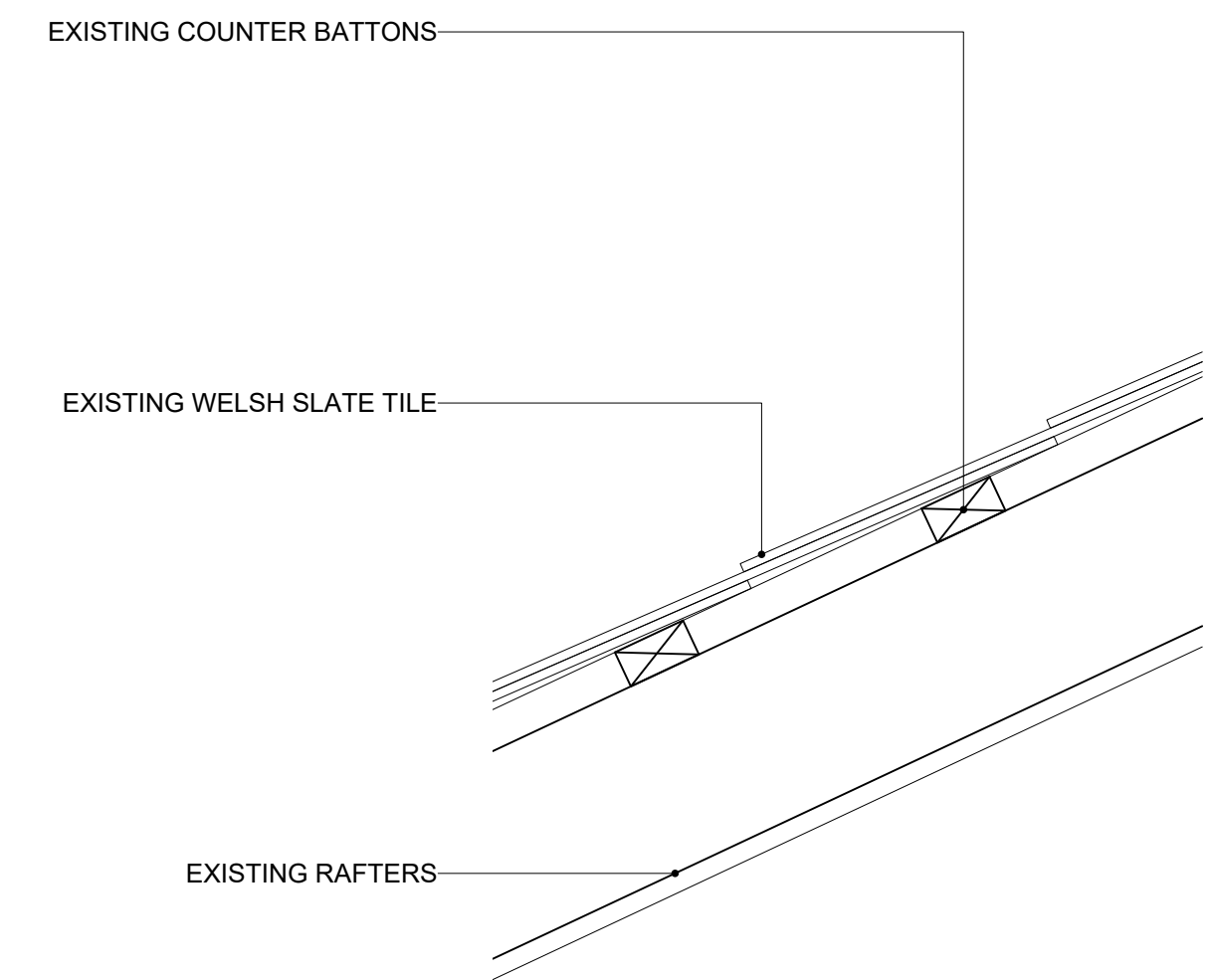
04 ROOF BUILD UP DETAIL 1:5 @ A1
