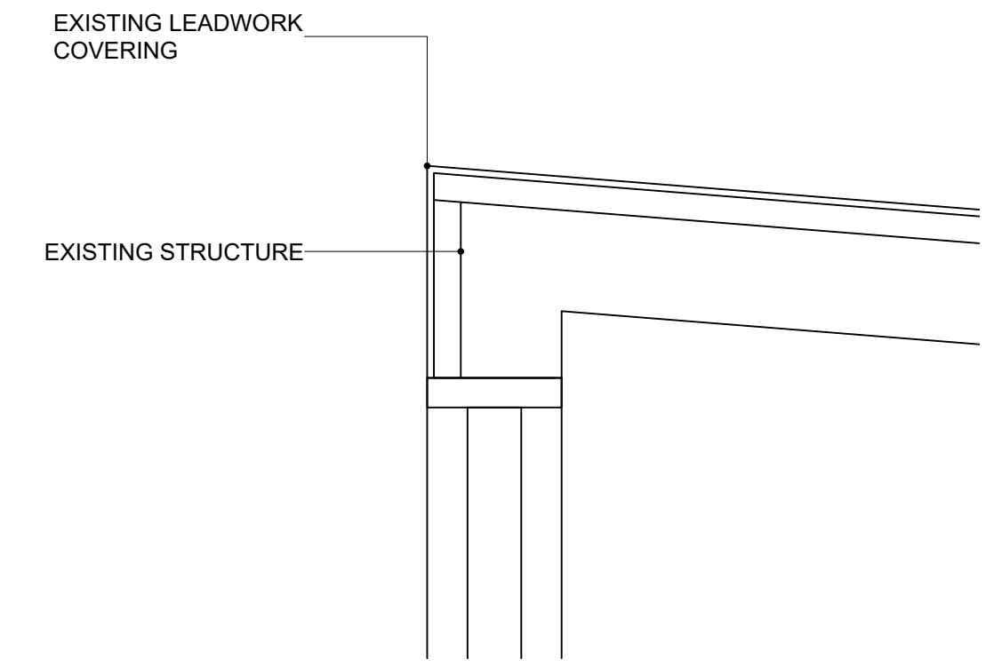
02 ACCESS HATCH BUILD UP DETAIL 1:5 @ A1
