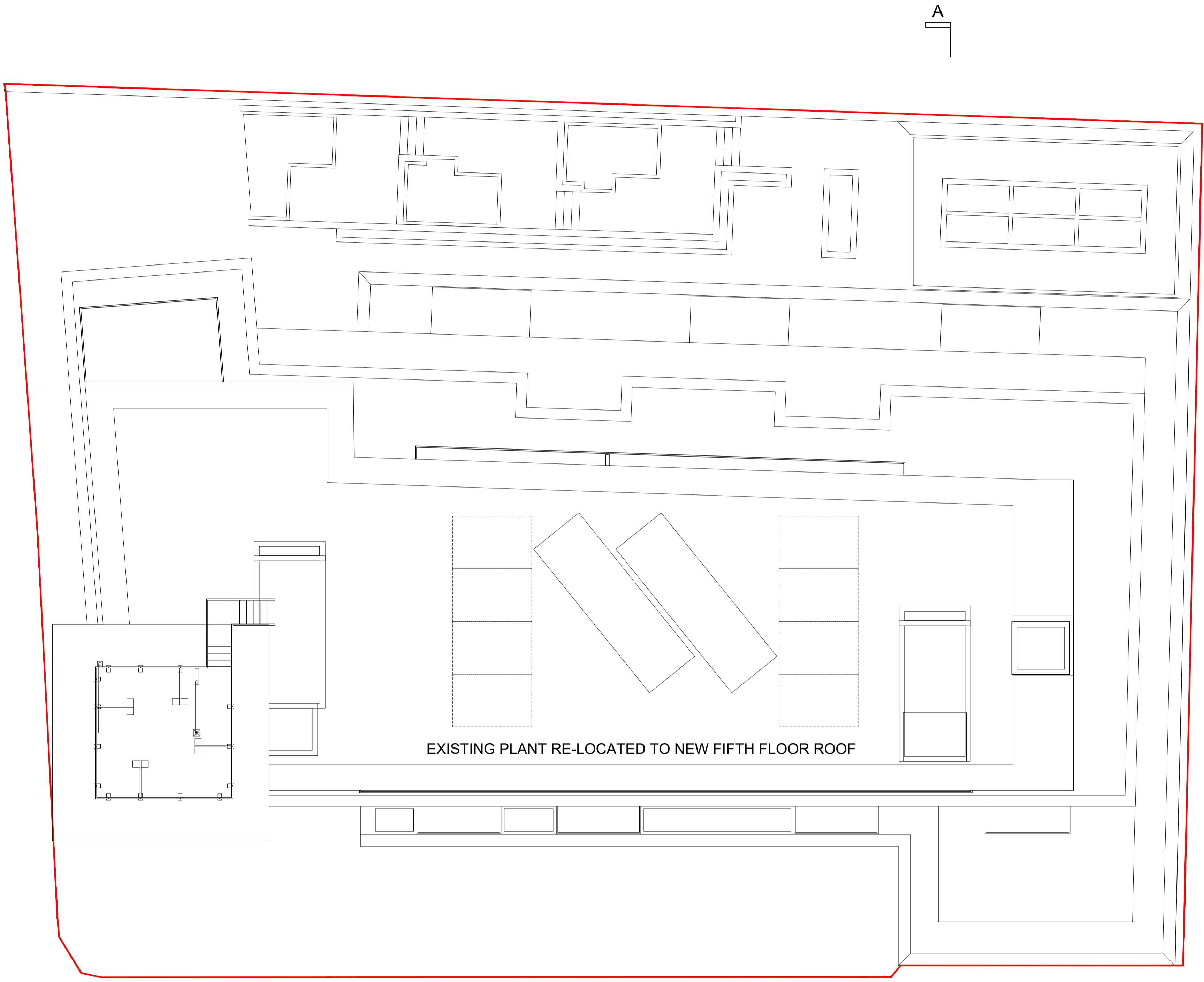
ROOF PLAN
