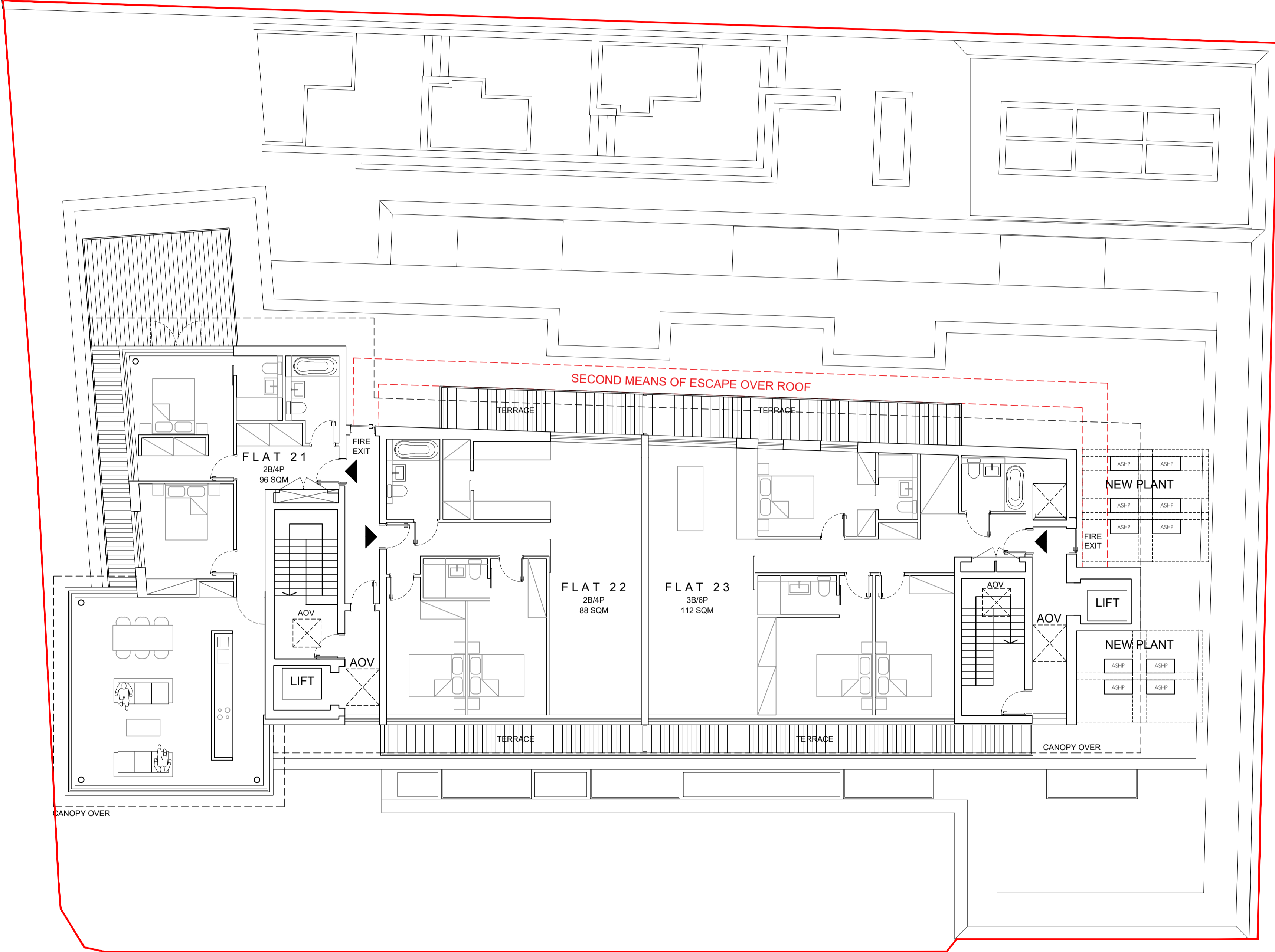
FIFTH FLOOR
