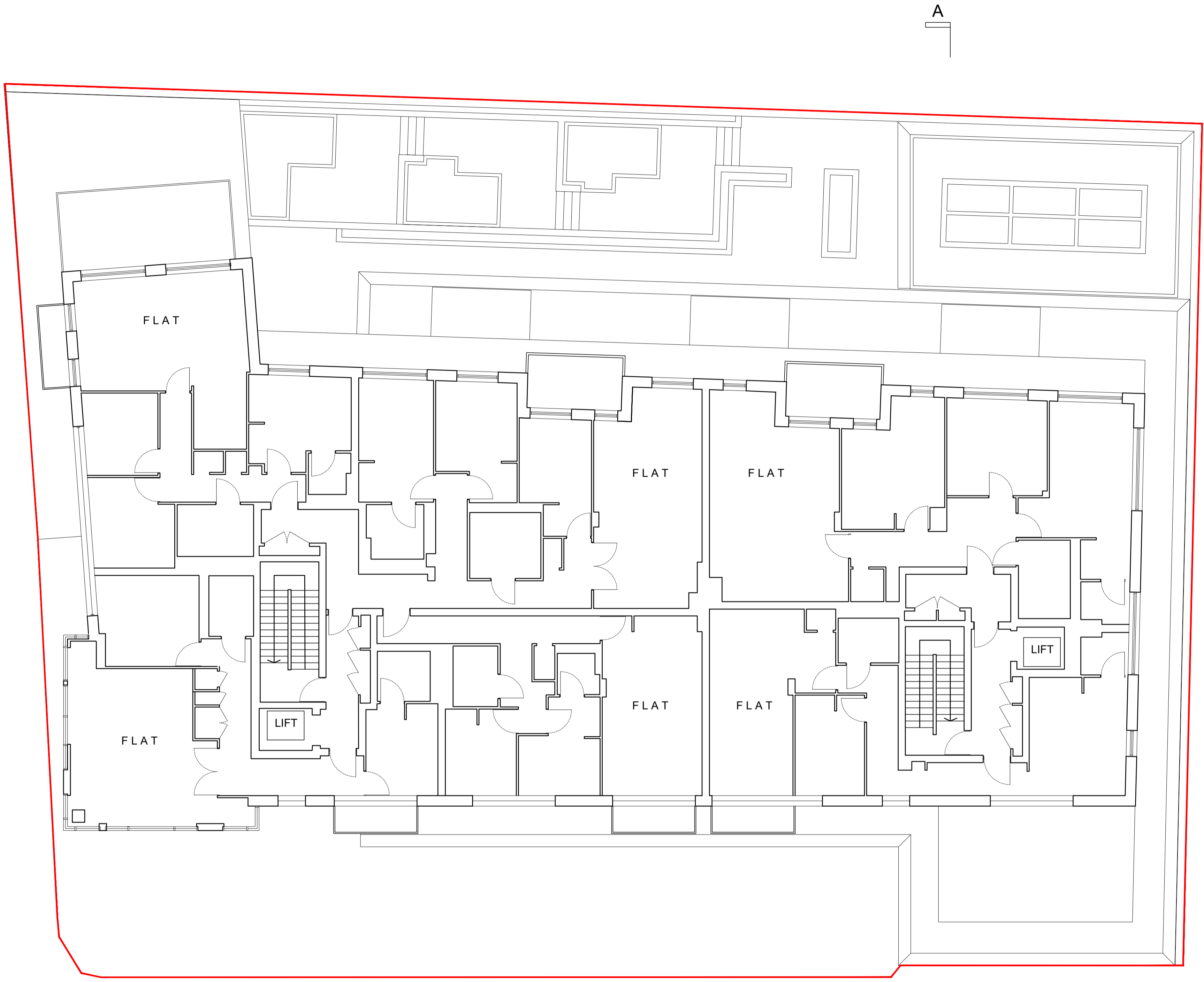
THIRD FLOOR
