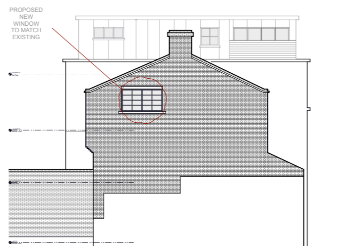
EXISTING SECTION B - 1:200@A3
