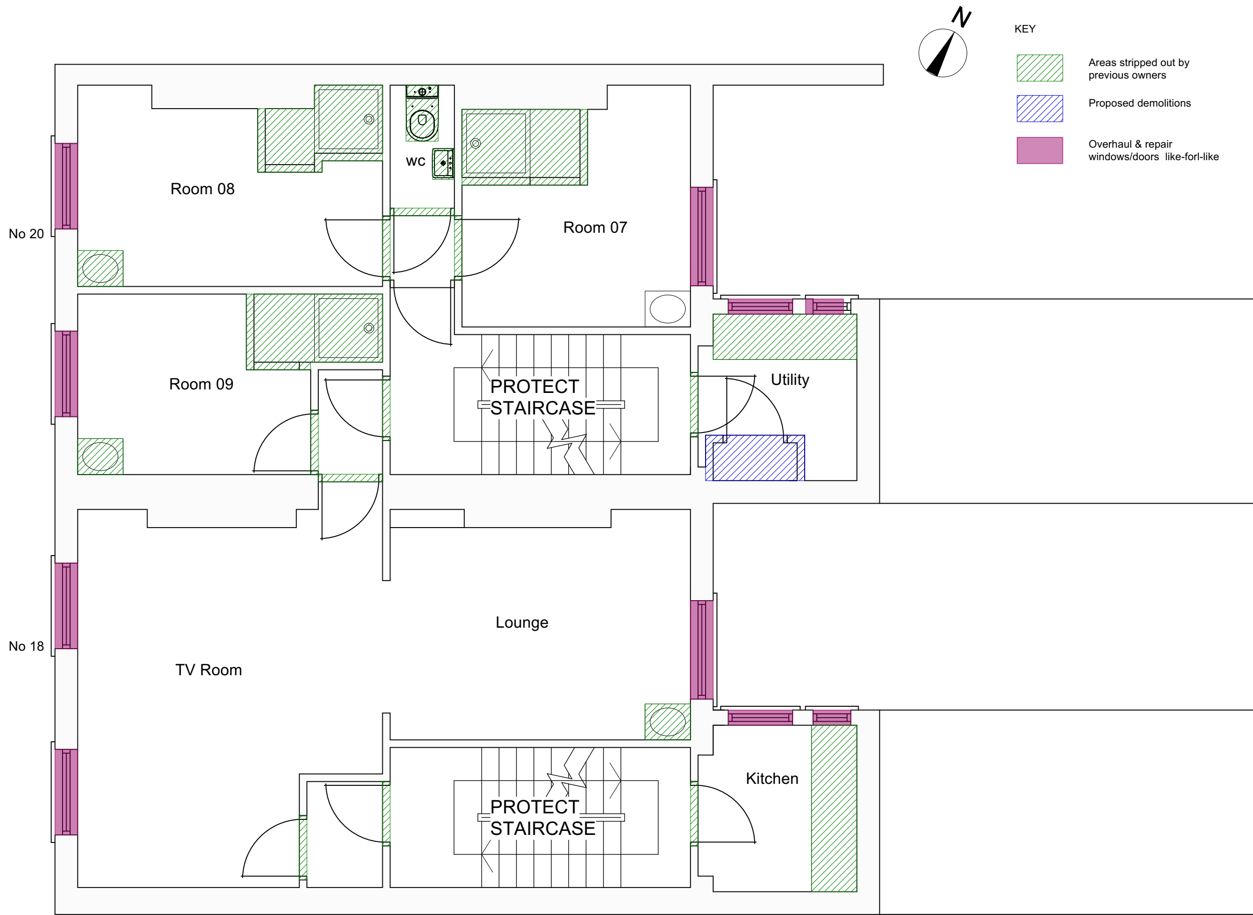
1 Demolition First Floor 103 Scale: 1:50
