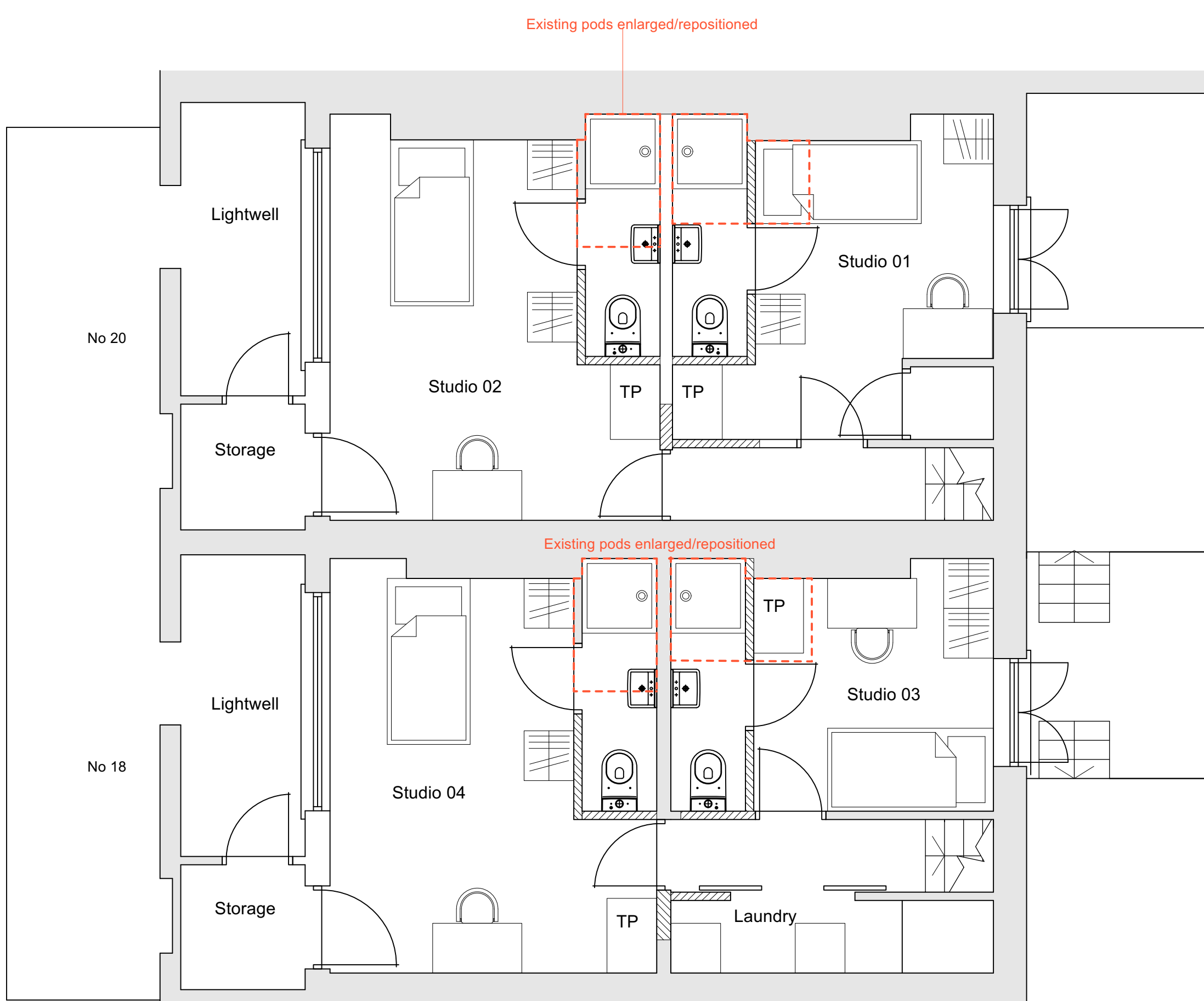
1 Proposed Basement 12 Scale: 1:50
