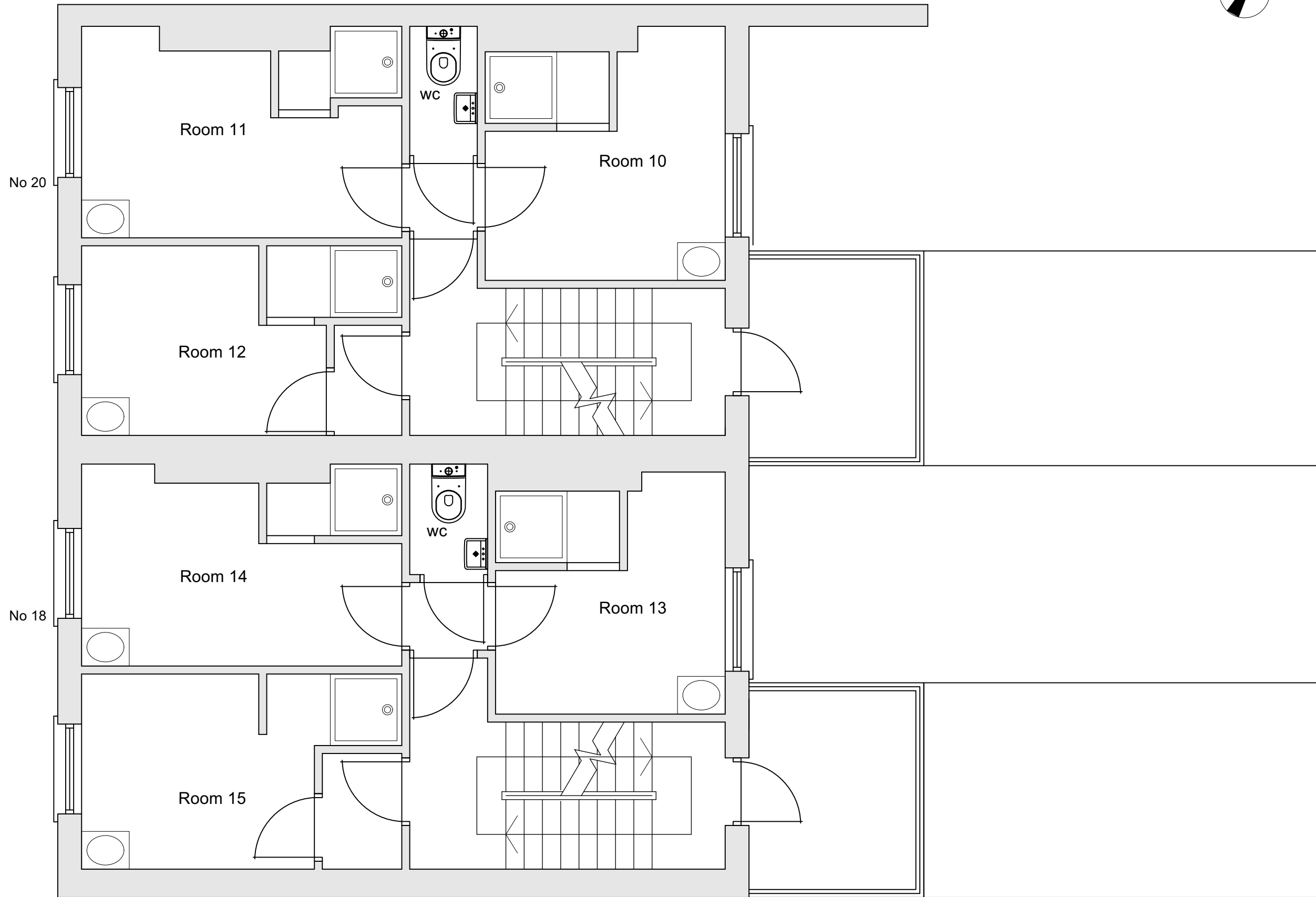
1 Existing Second Floor Plan 05 Scale: 1:50
