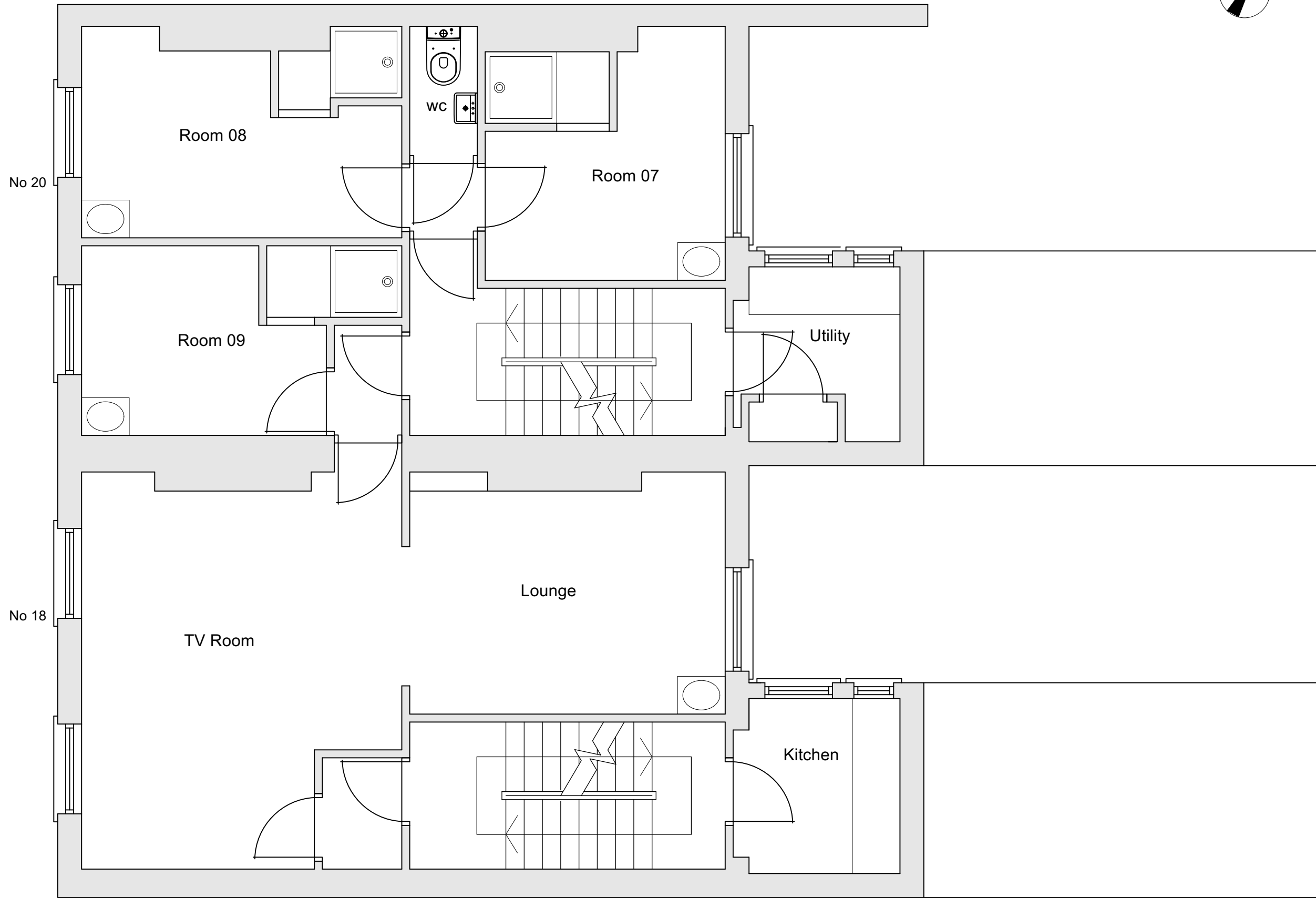
1 Existing First Floor Plan 04 Scale: 1:50
