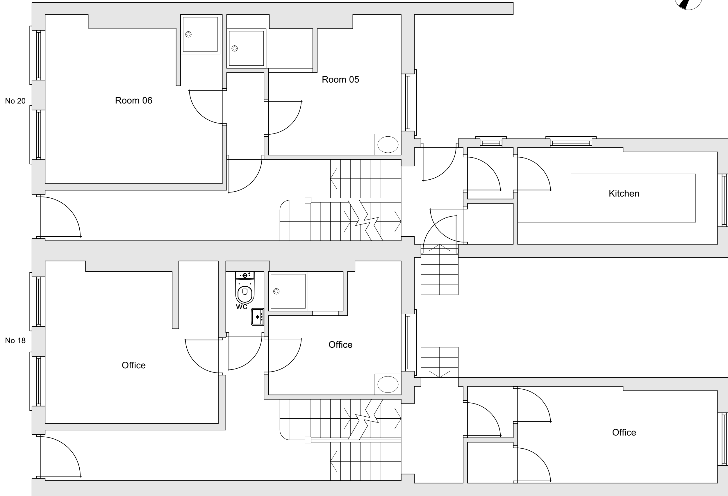
1 Existing Ground Floor Plan 03 Scale: 1:50
