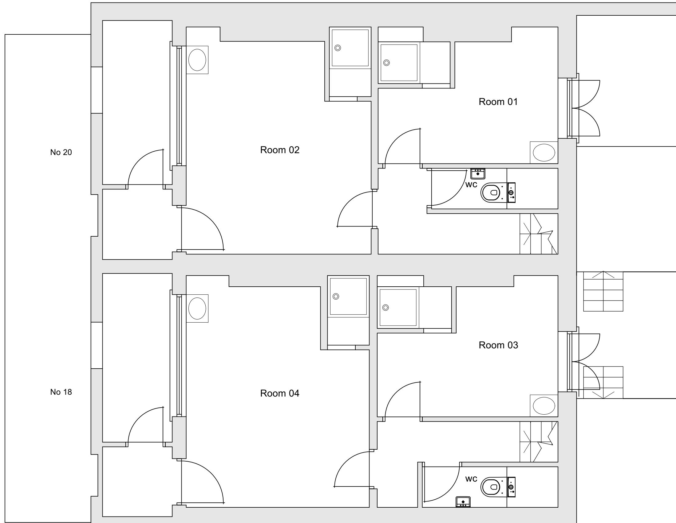
1 Existing Basement Plan 02 Scale: 1:50
