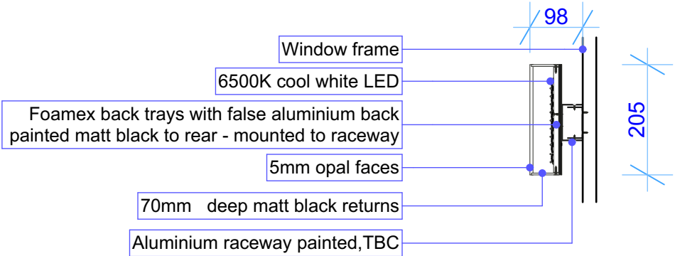
SECTION DETAIL
