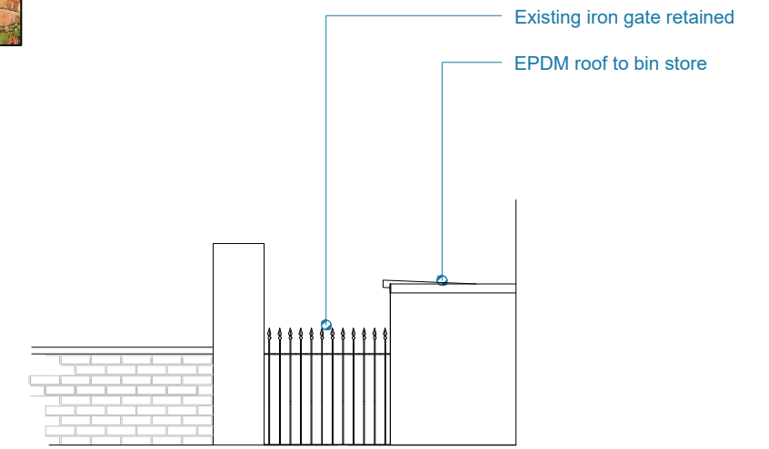
Section B
