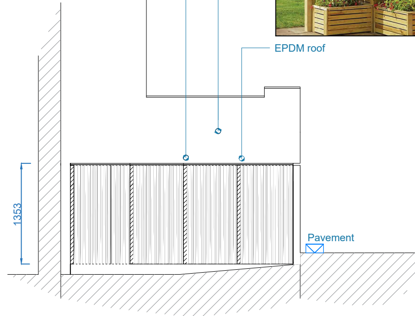
Section A
