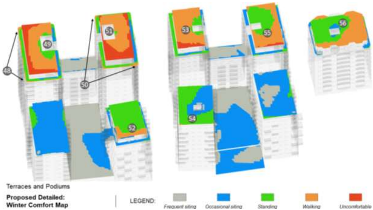
Figure 13.13 Proposed winter comfort map on Terraces and Podium (LCC), Detailed Proposals
