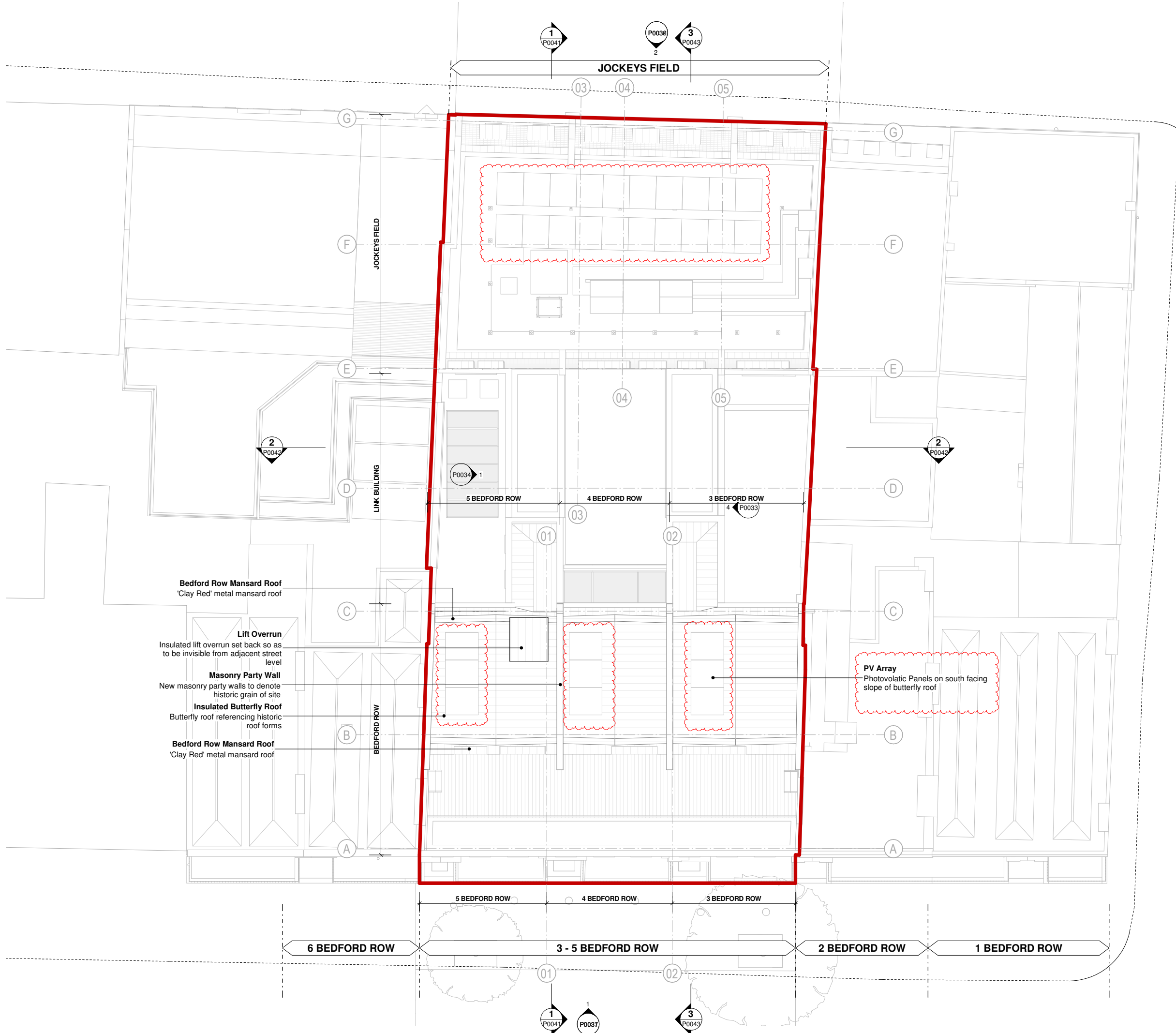
P0015 - E - Proposed Roof
