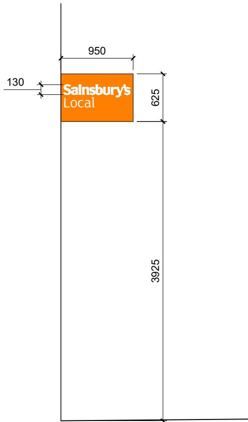
03 PROJECTING SIGNS P187574213 1:50@A3 ILLUMINATION LEVEL - 204 cd/m²
