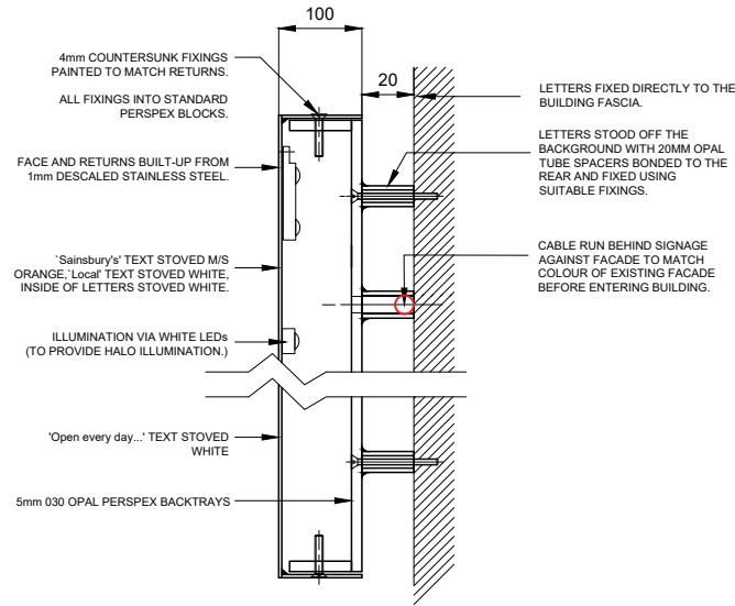
02 PROPOSED FASCIA SIGNAGE DETAILS P187574213 1:10@A3
