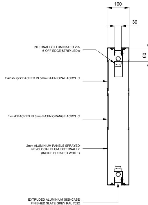
04 PROJECTING SIGN DETAIL P187574213 1:10@A3
