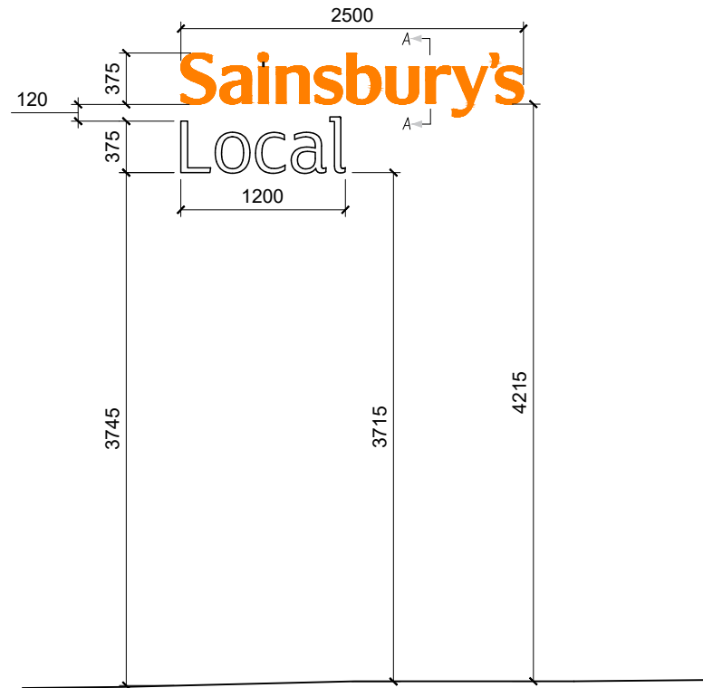
01 PROPOSED FASCIA SIGNAGE A - INTERNALLY ILLUMINATED- P187574213 1:50@A3 ILLUMINATION LEVEL - 375 cd/m²
