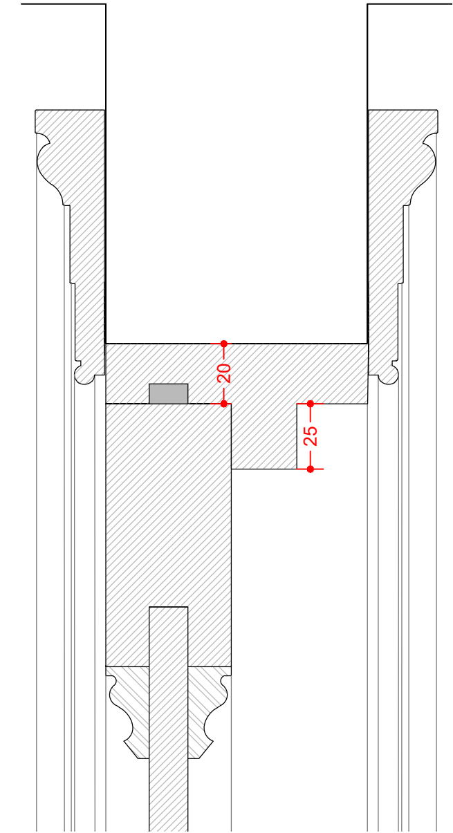
3 Door Head & Architrave Details Scale: 1:2
