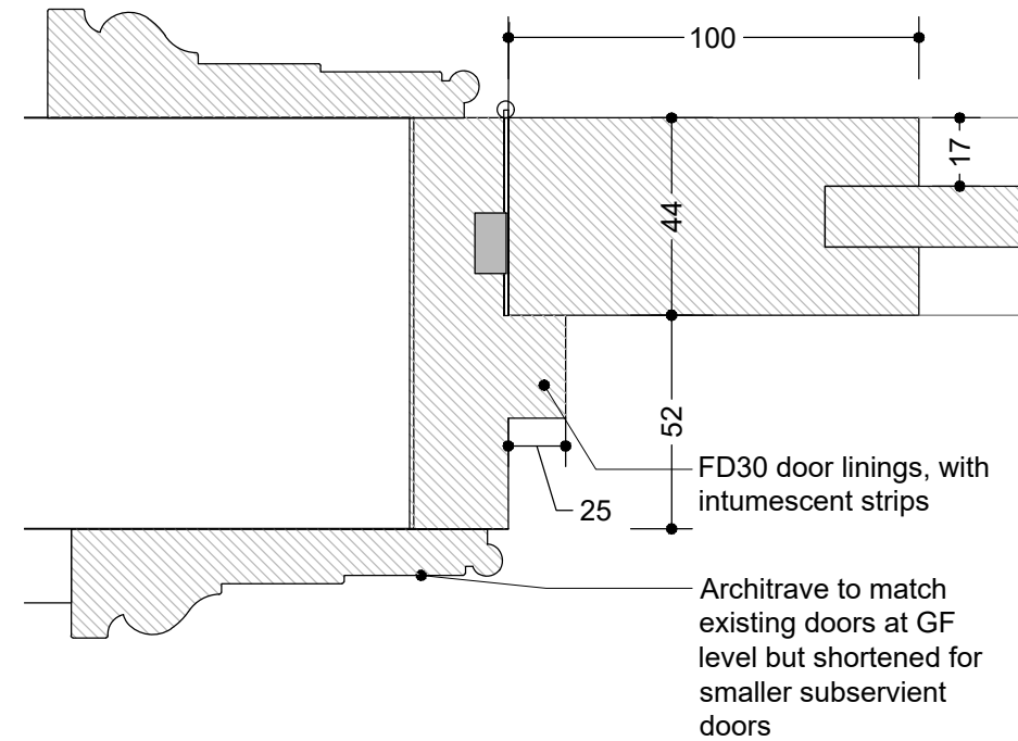
1 Door Lining and Architrave Scale: 1:2
