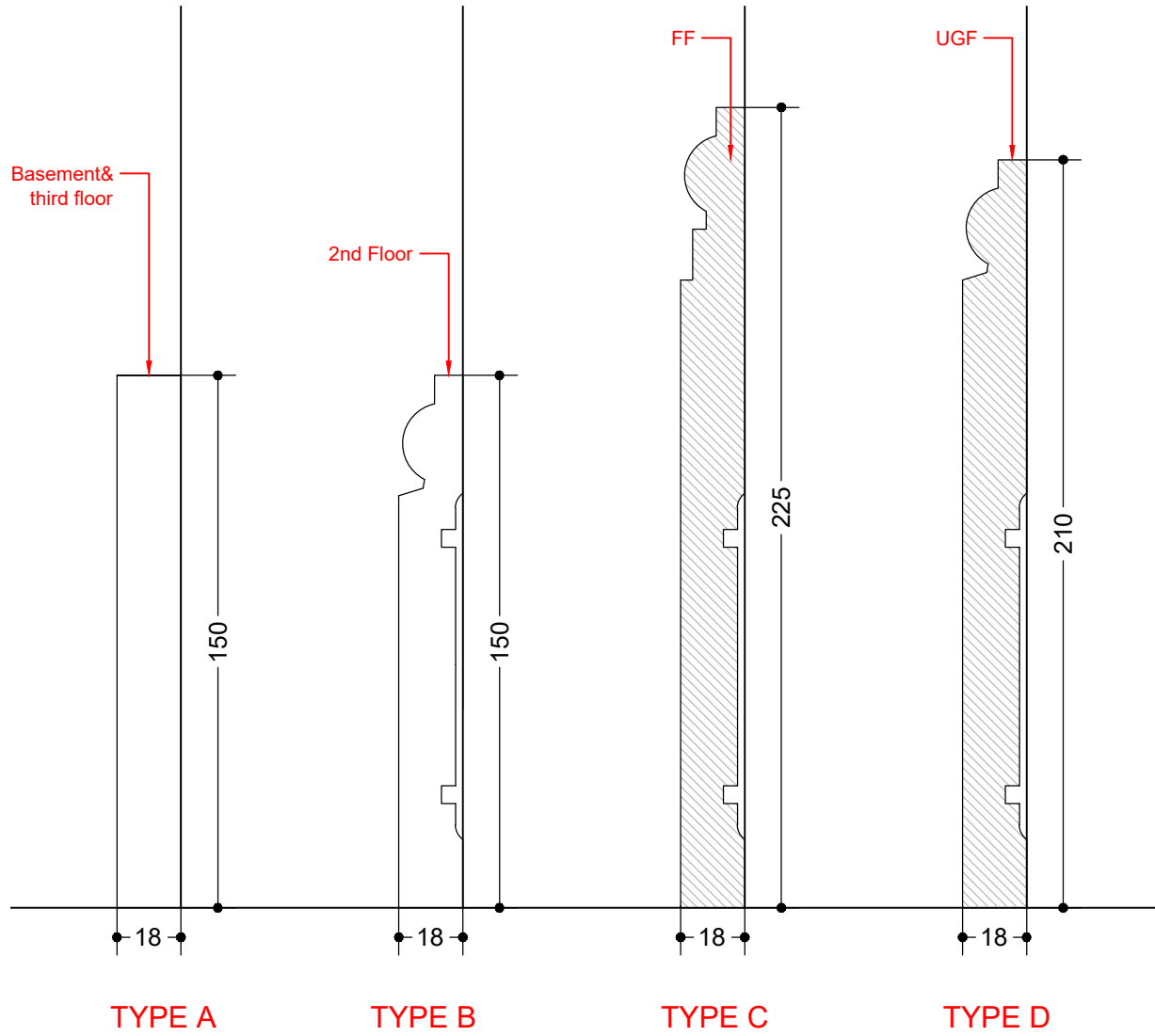
4 Skirting Detail Scale: 1:2
