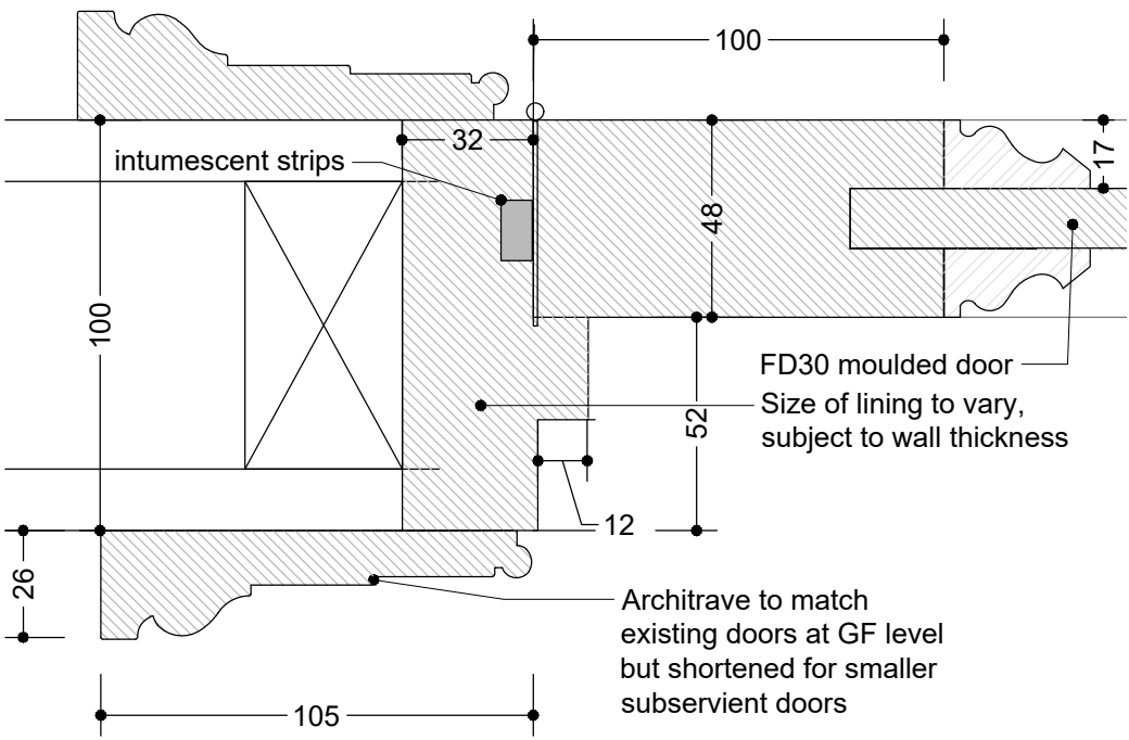
2 Door Lining and Architrave with Moulding Scale: 1:2
