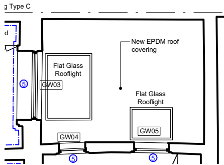
1 Ground Floor Plan Scale: 1:5
