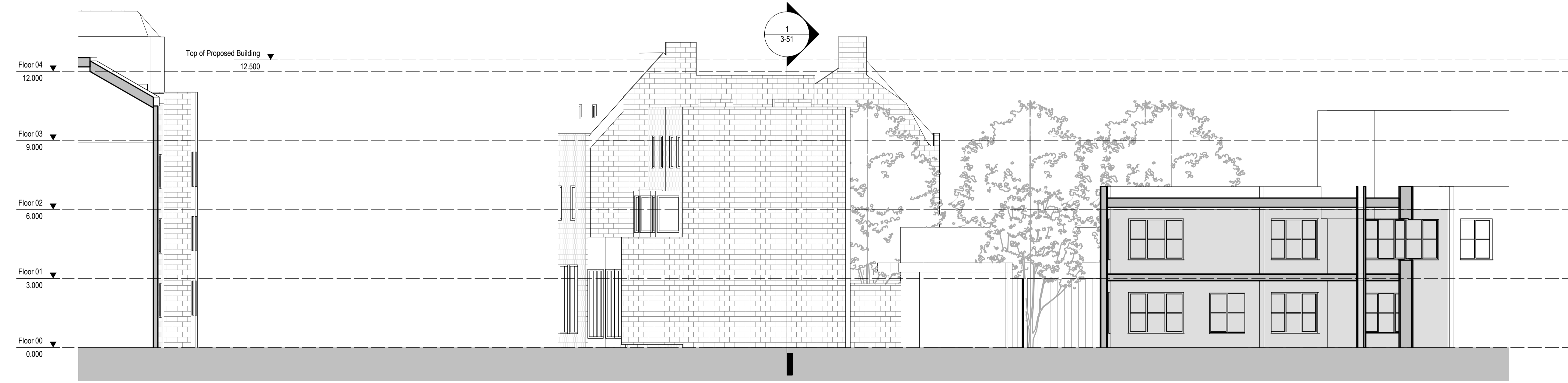
3 Section 3 Existing 1:100
