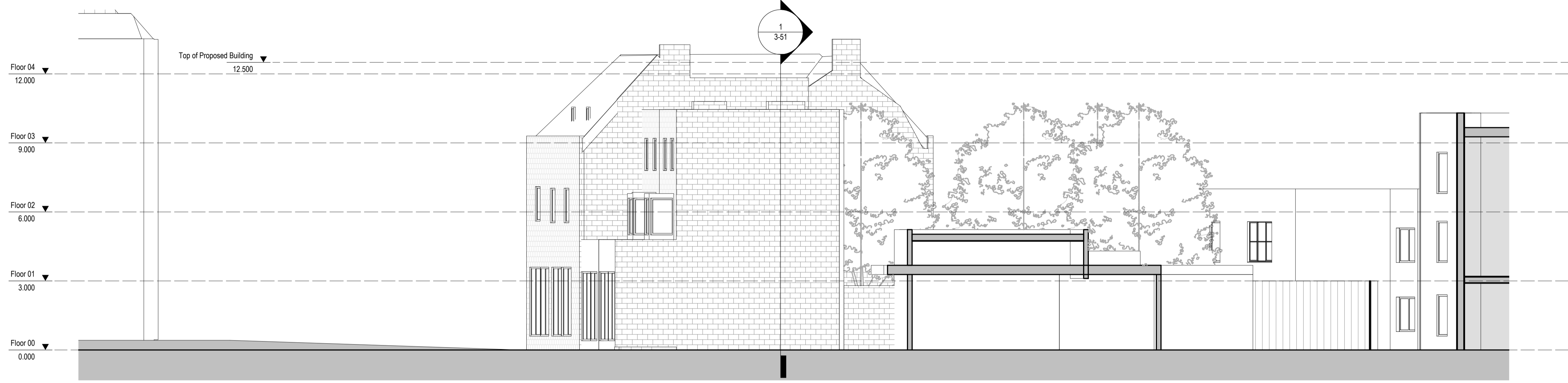
2 Section 2 Existing 1:100
