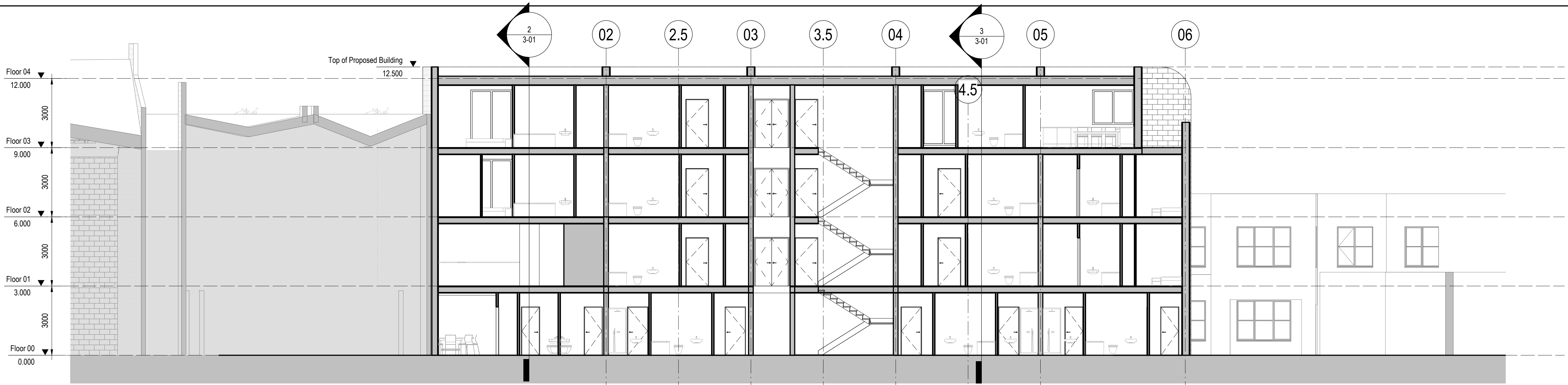
1 Section 1 1:100
