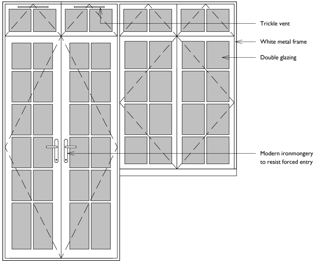
1 Proposed Type I 1 : 20
