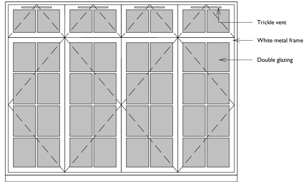
2 Proposed Type J 1 : 20
