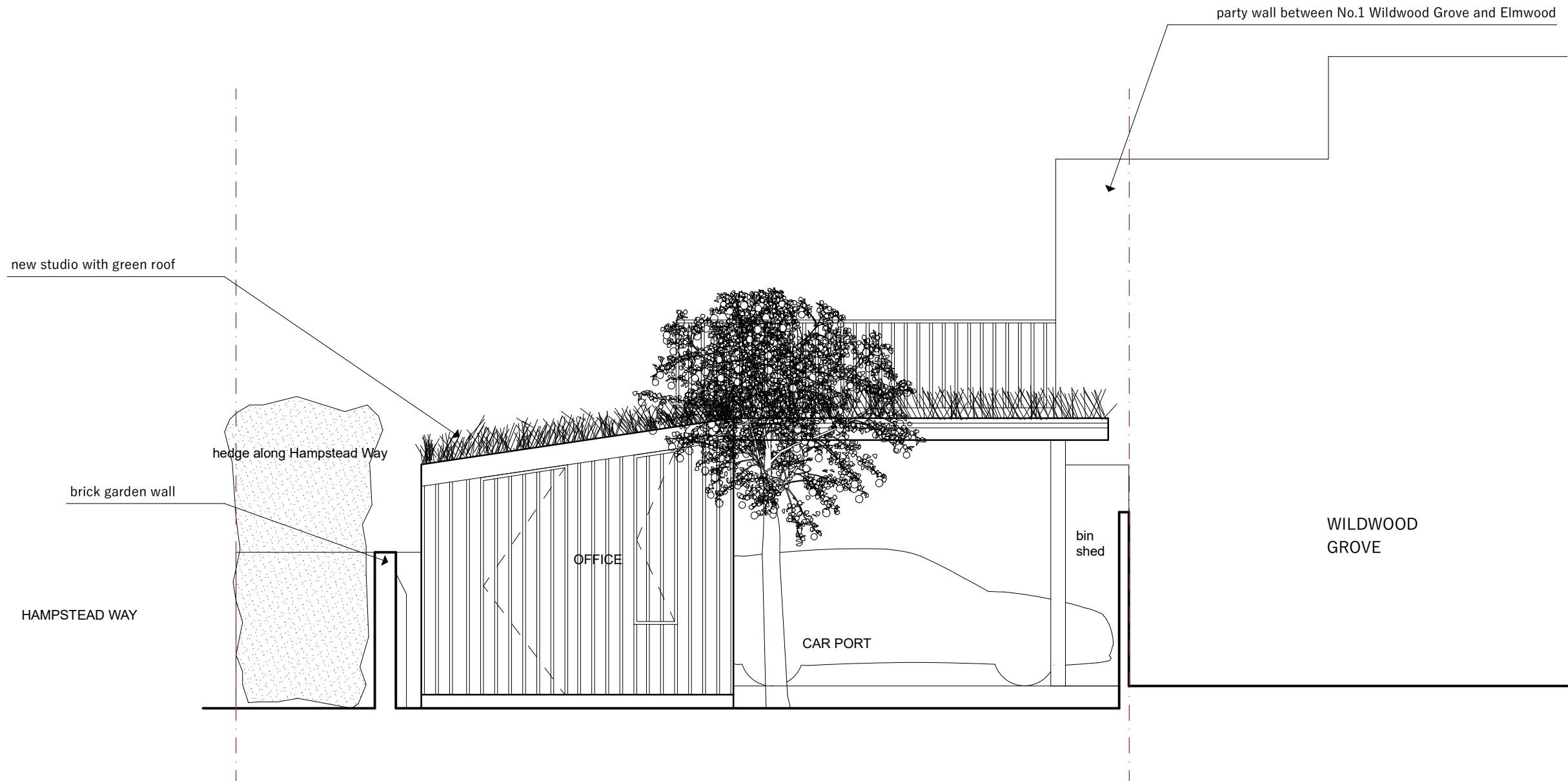
1 PROP SOUTH WEST REAR ELEVATION 1:50
