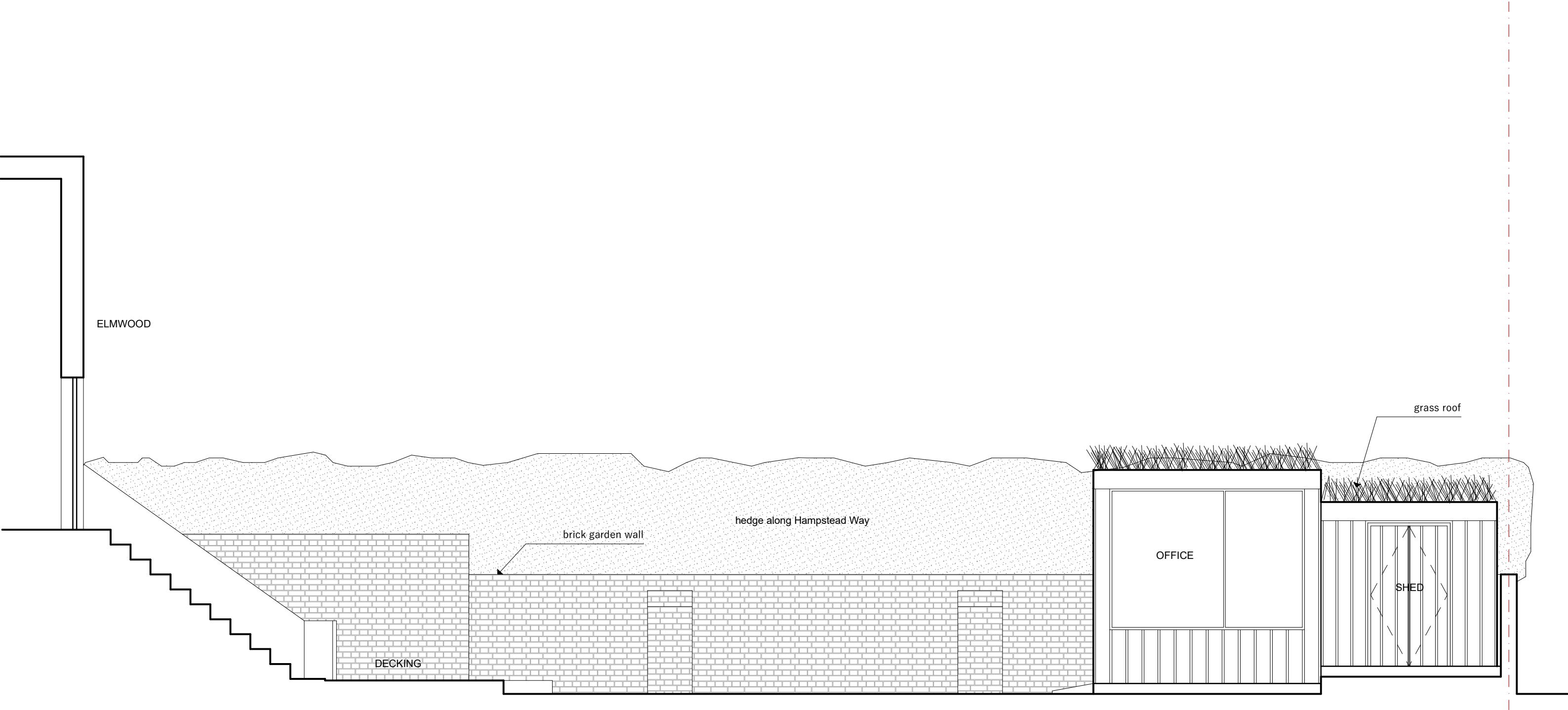
1 PROP SOUTH EAST SIDE ELEVATION 1:50
