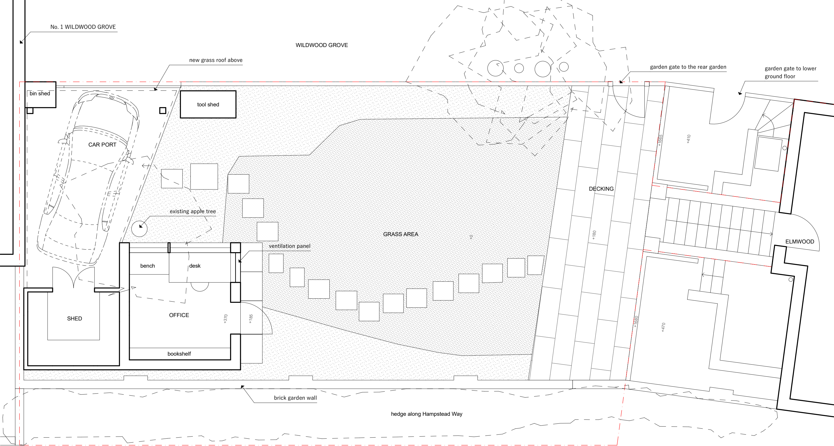
1 PROP GROUND FLOOR PLAN 1:50
