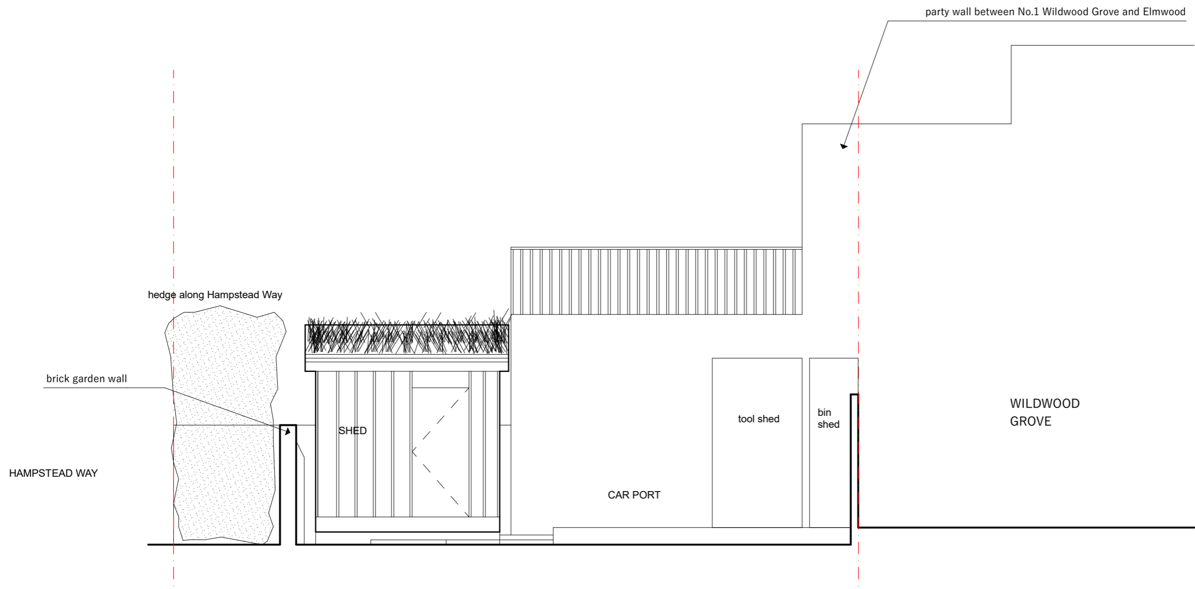
1 EXT SOUTH WEST REAR ELEVATION 1:50
