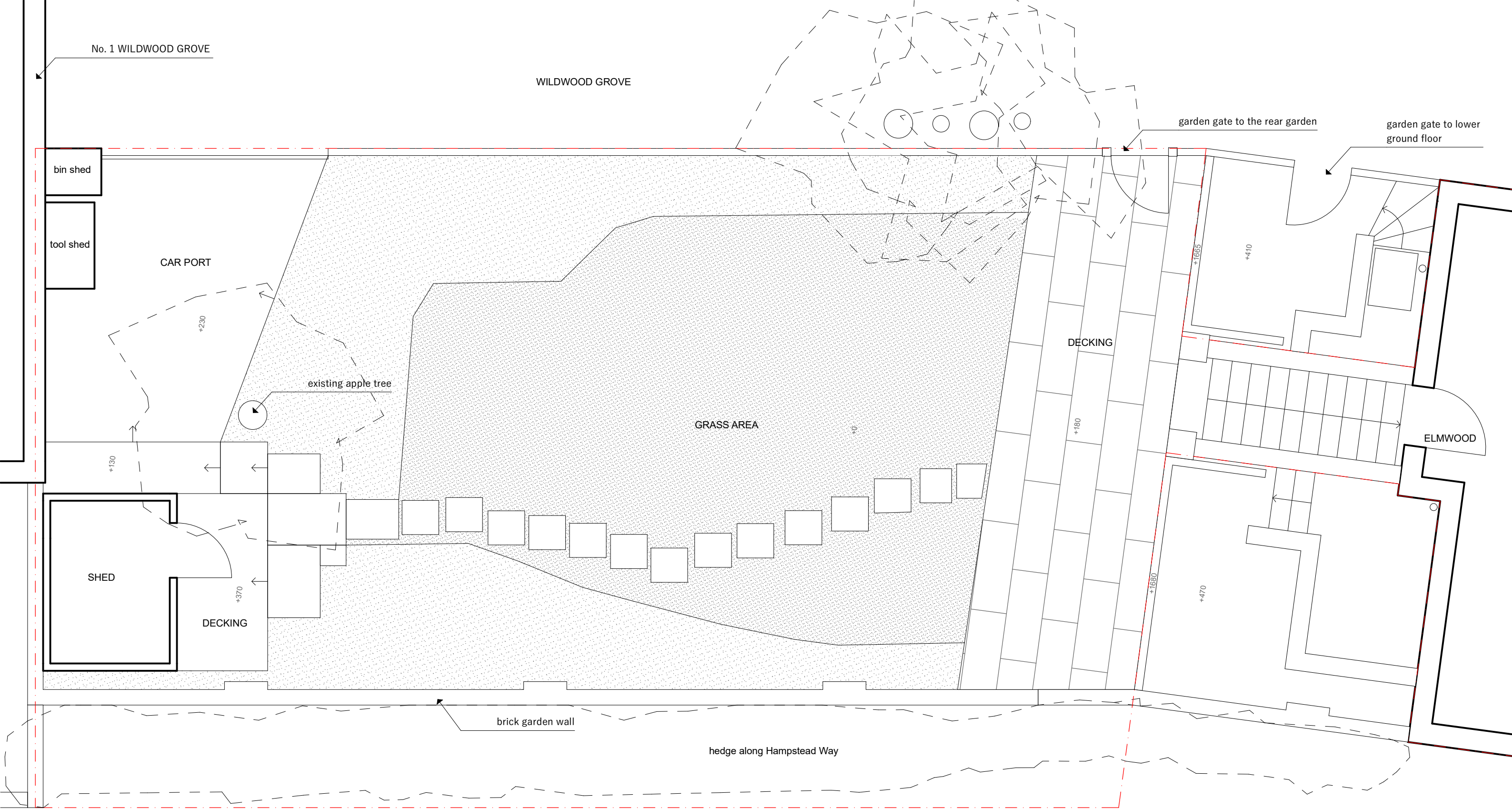
1 EXT GROUND FLOOR PLAN 1:50
