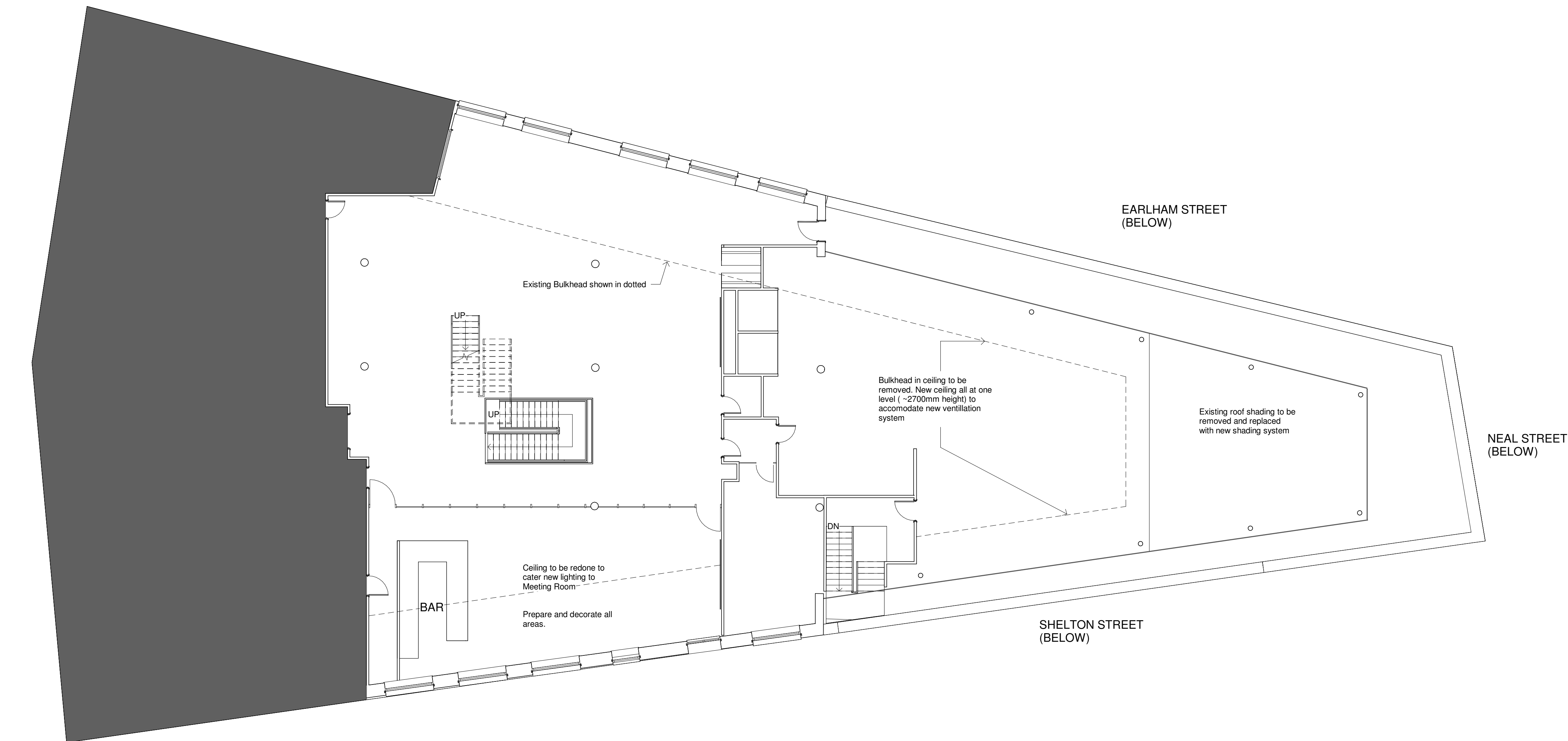
1 Existing/ Demo Plan - Fifth Floor 1 : 100
