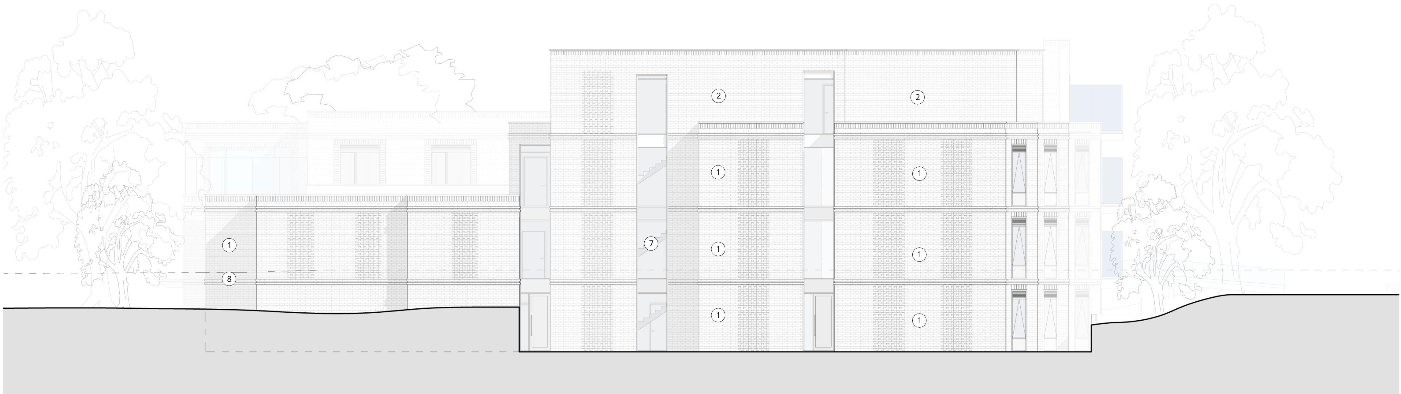
Proposed Eastern Elevation 1 : 100
