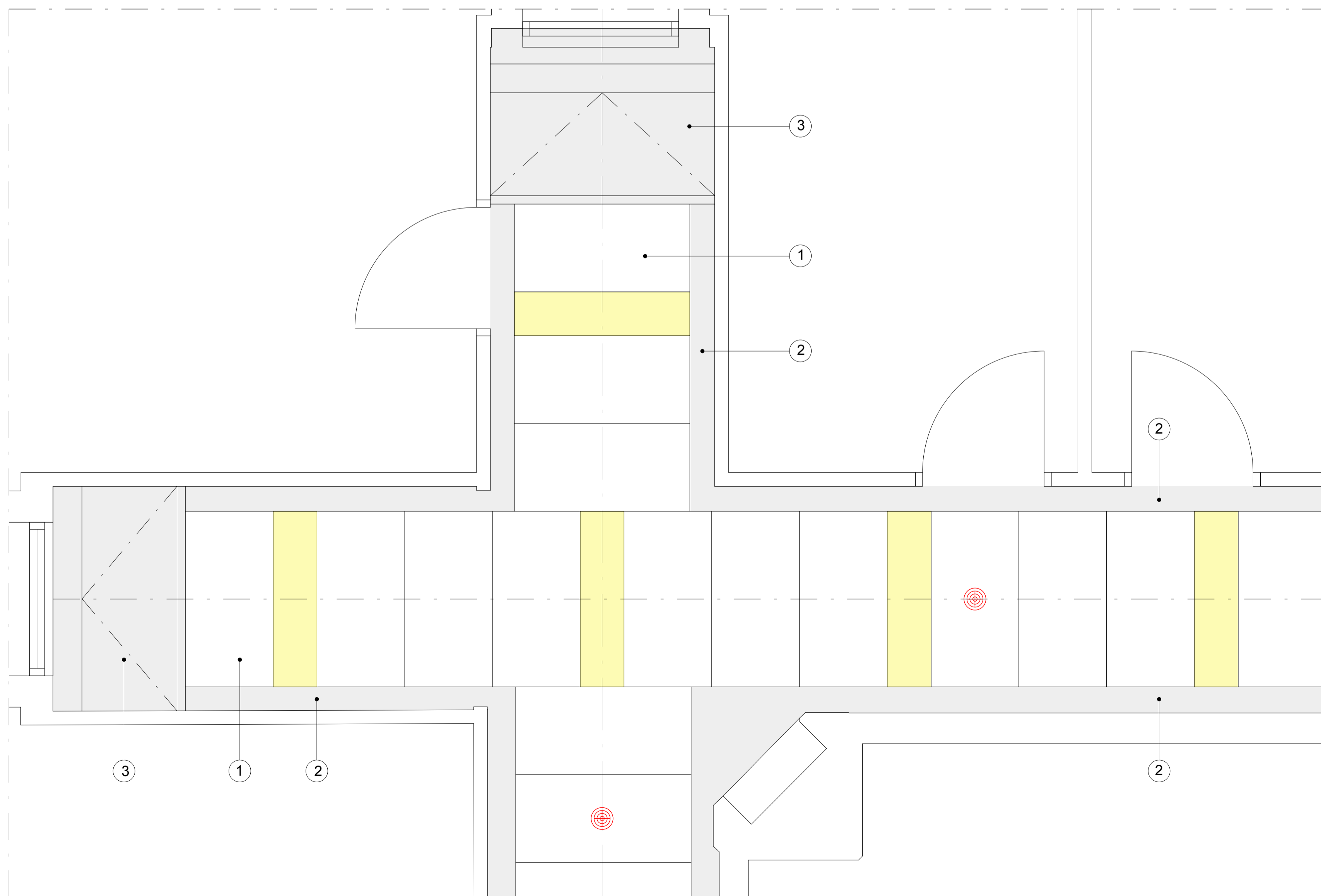
Proposed New Corridor Ceiling Plan - General Detail
